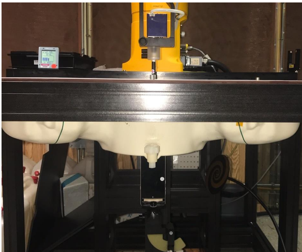
Figure 6-1 SAR measurement setup
