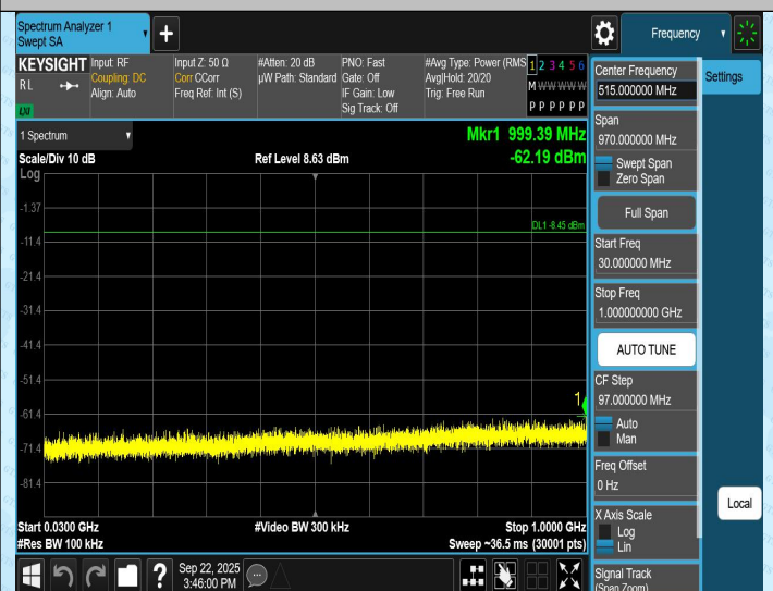
TX-Ant1-2472-30~1000-PASS
