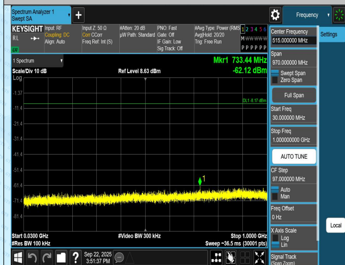
TX-Ant2-2472-30~1000-PASS
