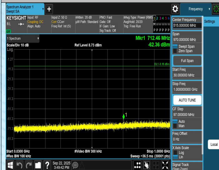
TX-Ant2-2440-30~1000-PASS
