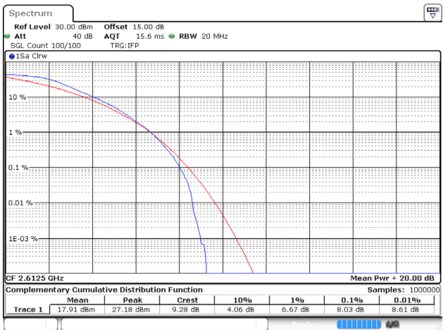
15MHz_High_QPSK_75@0
