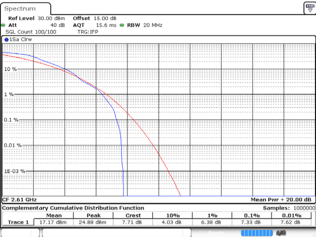
20MHz_High_QPSK_1@0
