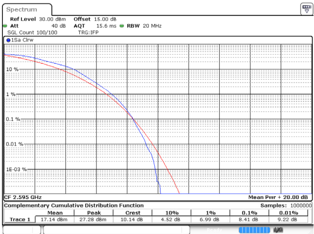
15MHz_Middle_16QAM_75@0
