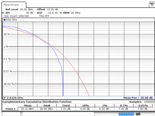
15MHz_High_QPSK_1@0
