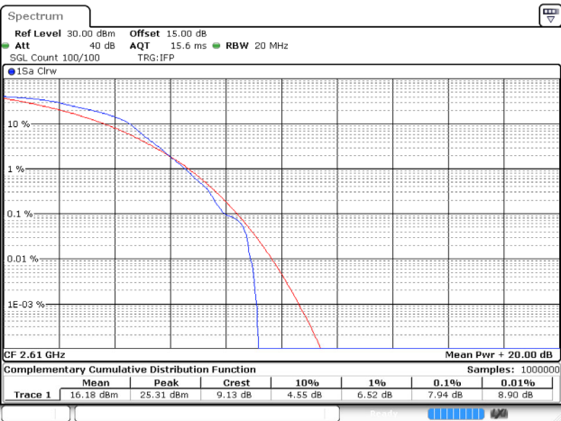
20MHz_High_16QAM_1@0
