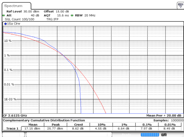
15MHz_High_16QAM_1@0
