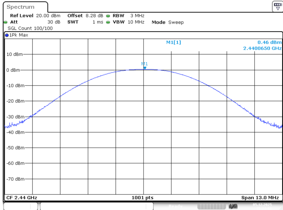
Power NVNT GFSK 2440MHz Ant1
