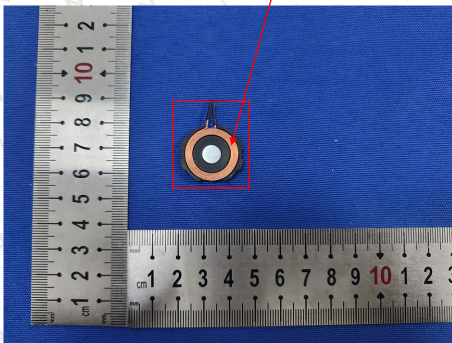
Coil Antenna-Watch
