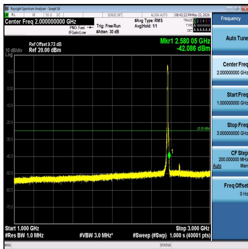
Band7-10MHz-16QAM-21400-50RB#0-1000~30 00-PASS
