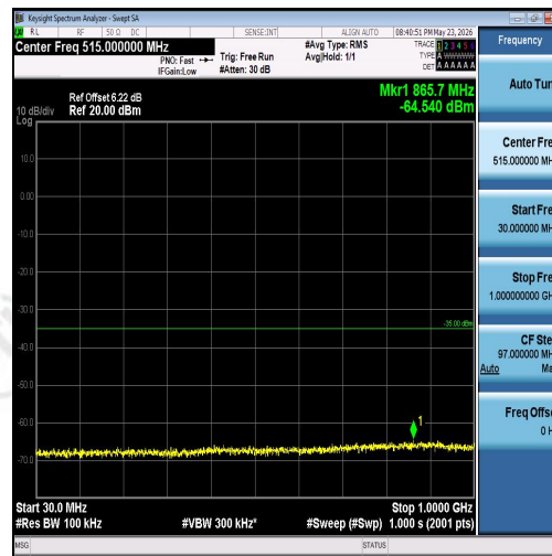
Band7-10MHz-QPSK-21400-50RB#0-30~1000-P ASS
