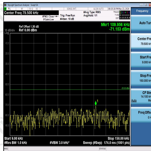
Band7-10MHz-QPSK-21400-1RB#0-0.009~0.15- PASS
