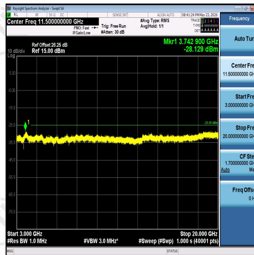
Band7-10MHz-QPSK-21400-50RB#0-3000~200 00-PASS
