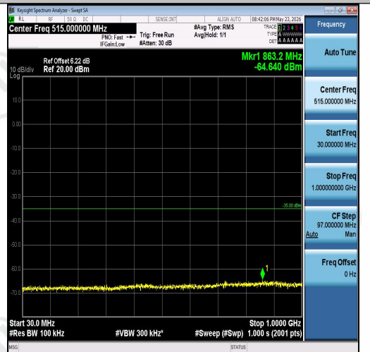
Band7-10MHz-16QAM-21400-50RB#0-30~1000- PASS
