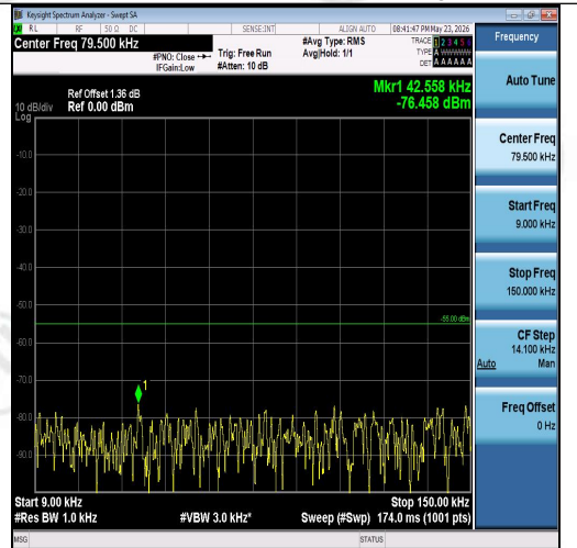
Band7-10MHz-16QAM-21400-50RB#0-0.009~0. 15-PASS
