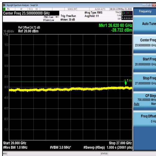
Band7-10MHz-16QAM-21100-50RB#0-20000~2 7000-PASS
