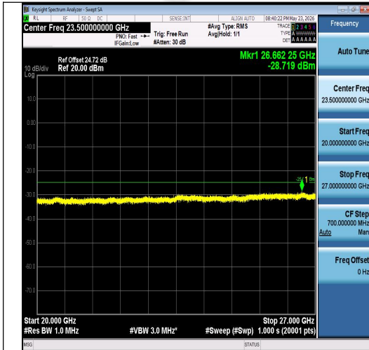
Band7-10MHz-16QAM-21400-1RB#49-20000~2 7000-PASS
