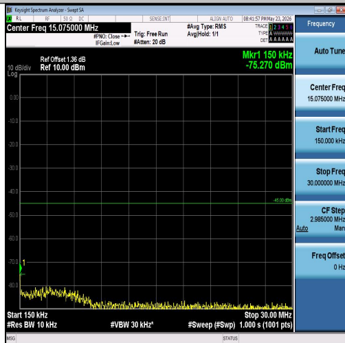
Band7-10MHz-16QAM-21400-50RB#0-0.15~30- PASS
