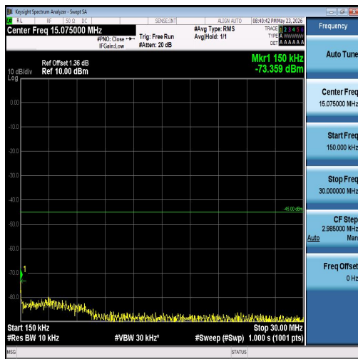
Band7-10MHz-QPSK-21400-50RB#0-0.15~30-P ASS
