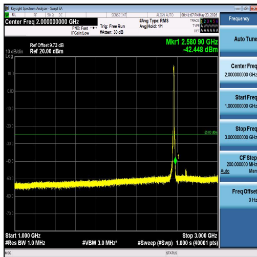
Band7-10MHz-QPSK-21400-50RB#0-1000~300 0-PASS
