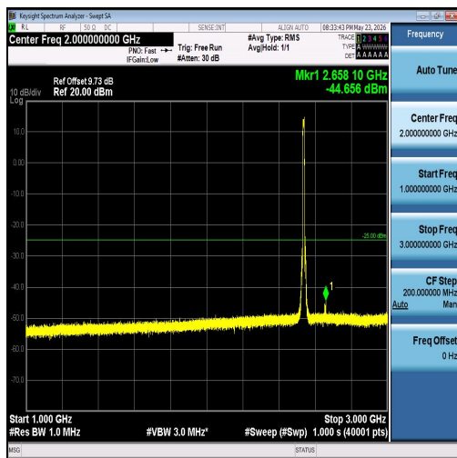
Band7-10MHz-16QAM-21100-50RB#0-1000~30 00-PASS
