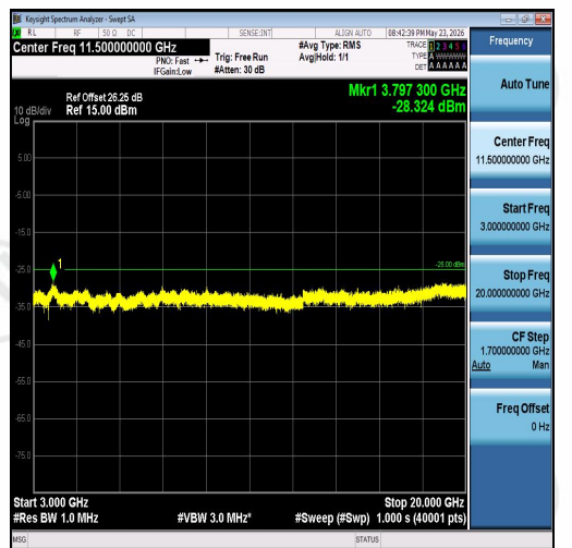
Band7-10MHz-16QAM-21400-50RB#0-3000~20 000-PASS
