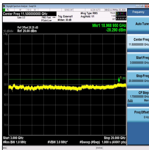
Band41-20MHz-16QAM-41490-1RB#99-3000~20000-PASS
