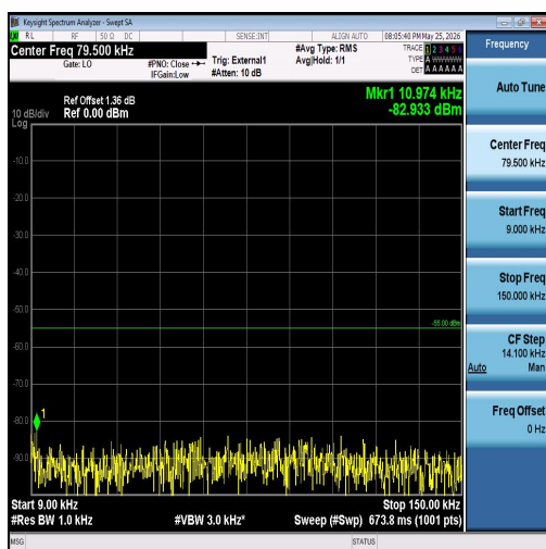
Band41-20MHz-16QAM-41490-100RB#0-0.009~0.15-PASS
