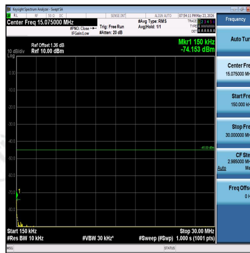
Band7-5MHz-16QAM-20775-25RB#0-0.15~30-P ASS
