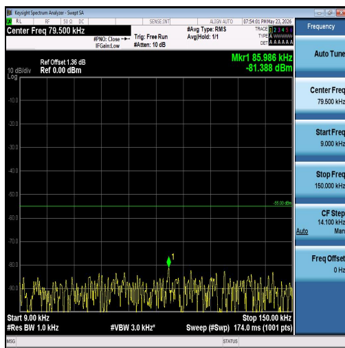
Band7-5MHz-16QAM-20775-25RB#0-0.009~0.1 5-PASS
