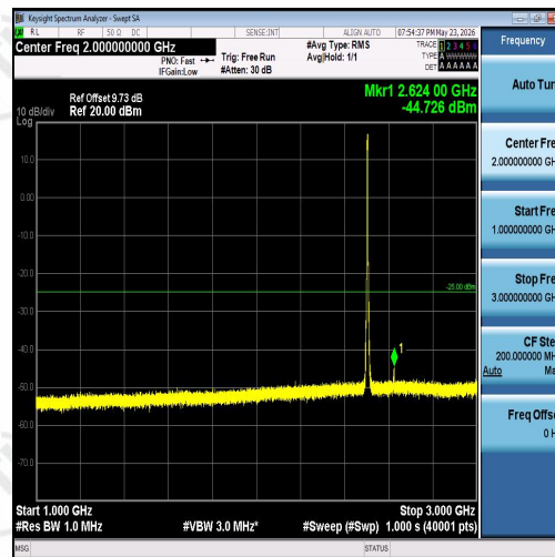
Band7-5MHz-16QAM-20775-25RB#0-1000~300 0-PASS
