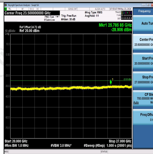
Band7-5MHz-16QAM-20775-25RB#0-20000~27
