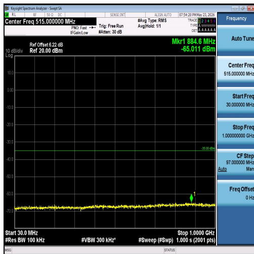
Band7-5MHz-16QAM-20775-25RB#0-30~1000-P ASS
