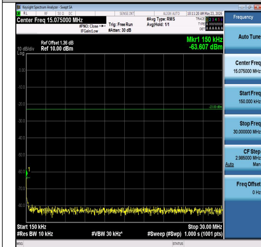
Band26(814-824)-5MHz-QPSK-26740-1RB#24-0 .15~30-PASS
