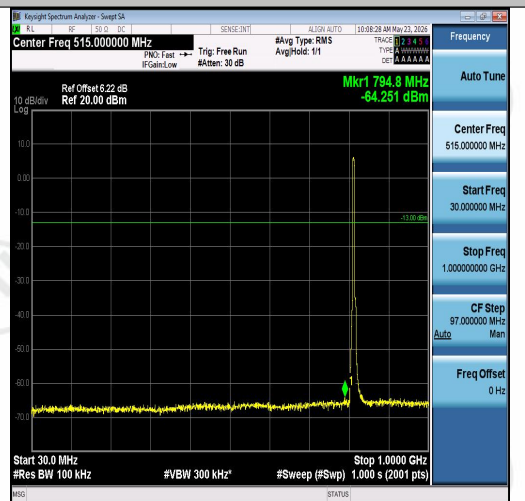
Band26(814-824)-5MHz-16QAM-26715-25RB#0 -30~1000-PASS
