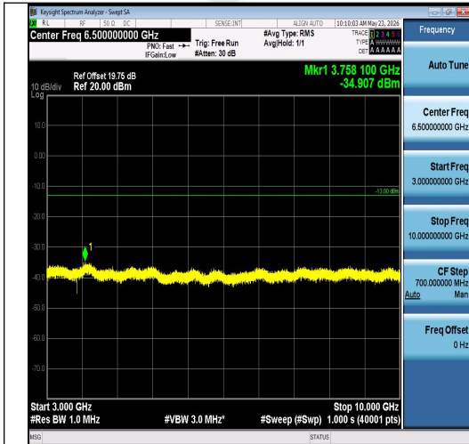
Band26(814-824)-5MHz-QPSK-26740-1RB#0-30 00~10000-PASS
