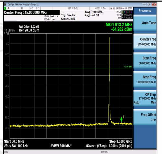
Band26(814-824)-5MHz-QPSK-26740-1RB#24-3 0~1000-PASS
