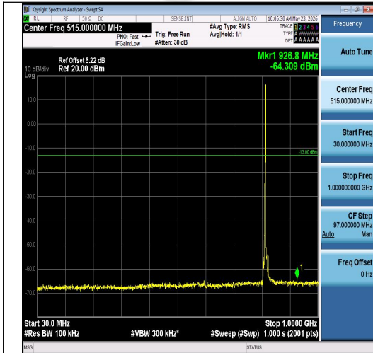
Band26(814-824)-5MHz-16QAM-26715-1RB#24 -30~1000-PASS
