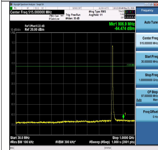
Band26(814-824)-5MHz-QPSK-26740-25RB#0-3 0~1000-PASS
