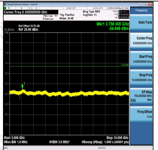
Band26(814-824)-5MHz-16QAM-26715-1RB#0-3000~10000-PASS
