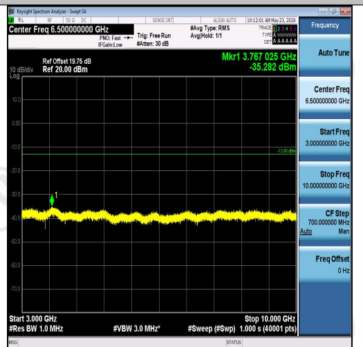
Band26(814-824)-5MHz-QPSK-26740-1RB#24-3 000~10000-PASS
