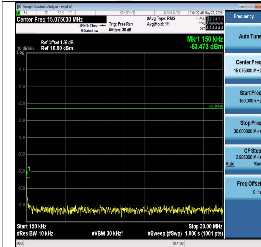
Band26(814-824)-5MHz-16QAM-26715-1RB#0-0.15~30-PASS
