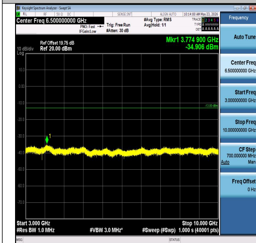
Band26(814-824)-5MHz-QPSK-26740-25RB#0-3 000~10000-PASS
