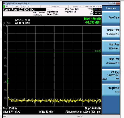
Band26(814-824)-5MHz-QPSK-26740-1RB#0-0. 15~30-PASS
