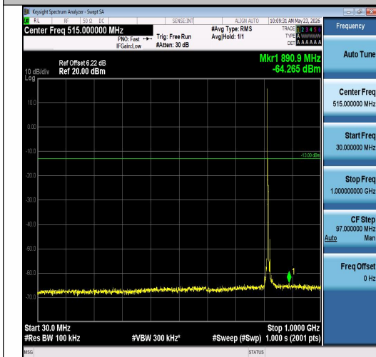
Band26(814-824)-5MHz-QPSK-26740-1RB#0-30 ~1000-PASS
