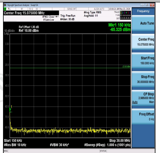
Band26(814-824)-5MHz-16QAM-26715-1RB#24-0.15~30-PASS
