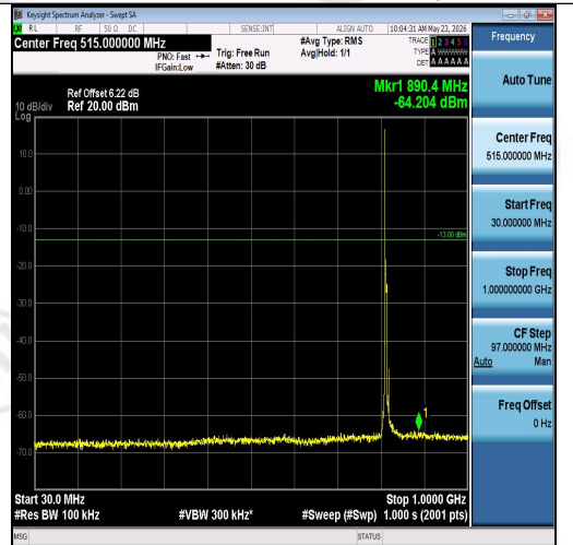
Band26(814-824)-5MHz-16QAM-26715-1RB#0-30~1000-PASS
