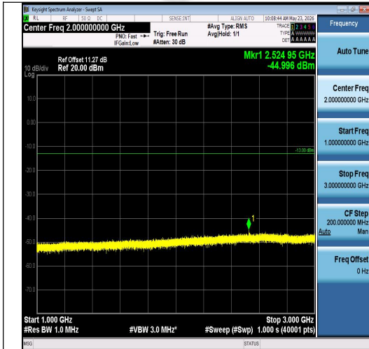
Band26(814-824)-5MHz-16QAM-26715-25RB#0 -1000~3000-PASS
