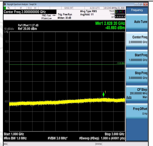
Band26(814-824)-5MHz-QPSK-26740-25RB#0-1 000~3000-PASS
