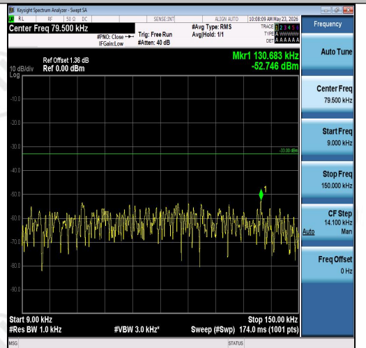
Band26(814-824)-5MHz-16QAM-26715-25RB#0 -0.009~0.15-PASS
