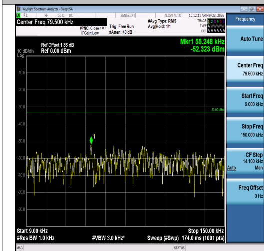
Band26(814-824)-5MHz-16QAM-26740-1RB#24-0.009~0.15-PASS
