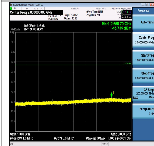
Band26(814-824)-5MHz-QPSK-26740-1RB#24-1 000~3000-PASS
