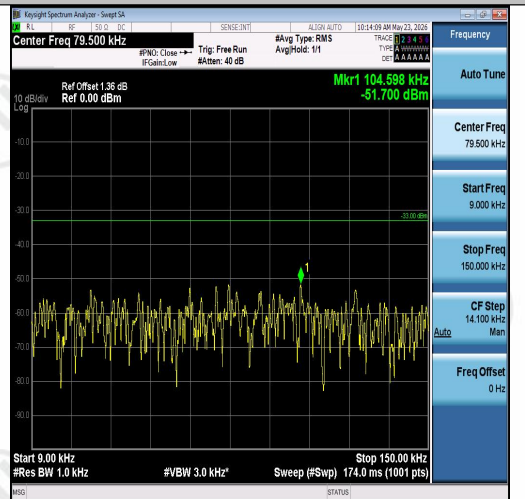
Band26(814-824)-5MHz-16QAM-26740-25RB#0 -0.009~0.15-PASS
