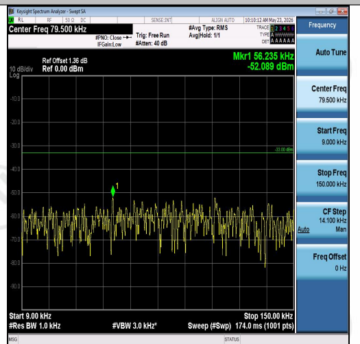
Band26(814-824)-5MHz-16QAM-26740-1RB#0-0 0.009~0.15-PASS
