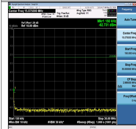
Band26(814-824)-5MHz-16QAM-26740-25RB#0 -0.15~30-PASS
