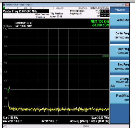
Band26(814-824)-5MHz-16QAM-26740-1RB#24-0.15~30-PASS
