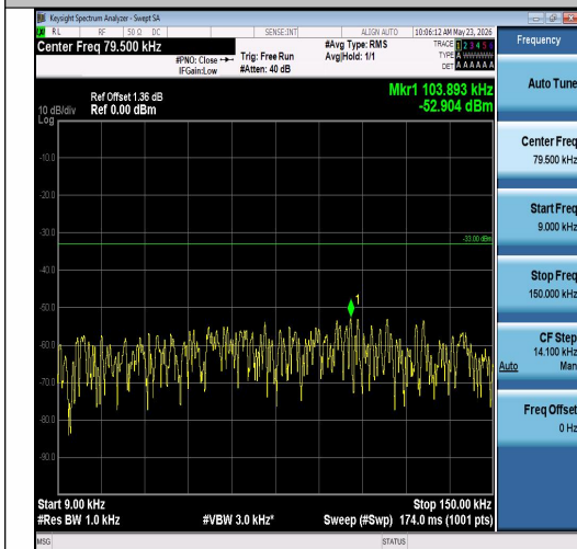
Band26(814-824)-5MHz-16QAM-26715-1RB#24-0.009~0.15-PASS
