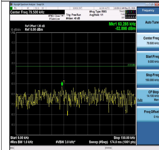
Band26(814-824)-5MHz-QPSK-26740-1RB#0-0. 009~0.15-PASS
