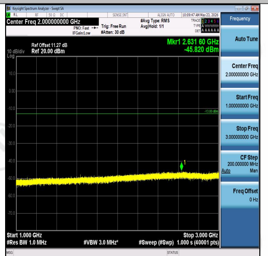
Band26(814-824)-5MHz-QPSK-26740-1RB#0-10 00~3000-PASS
