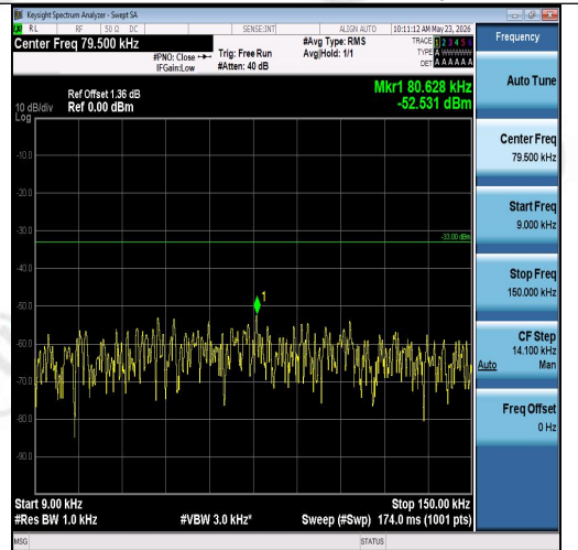
Band26(814-824)-5MHz-QPSK-26740-1RB#24-0 .009~0.15-PASS
