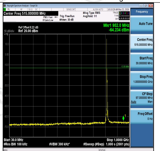
Band26(814-824)-5MHz-16QAM-26740-1RB#0-30~1000-PASS
