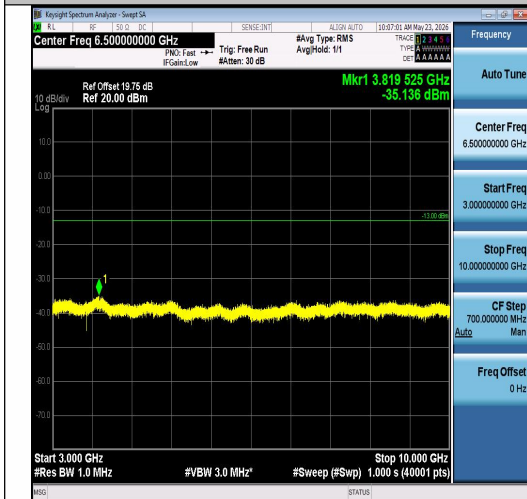
Band26(814-824)-5MHz-16QAM-26715-1RB#24 -3000~10000-PASS
