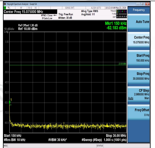
Band26(814-824)-5MHz-QPSK-26740-25RB#0-0 .15~30-PASS
