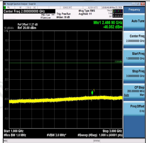
Band26(814-824)-5MHz-16QAM-26715-1RB#24 -1000~3000-PASS
