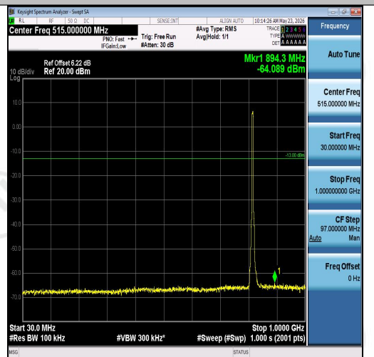
Band26(814-824)-5MHz-16QAM-26740-25RB#0 -30~1000-PASS
