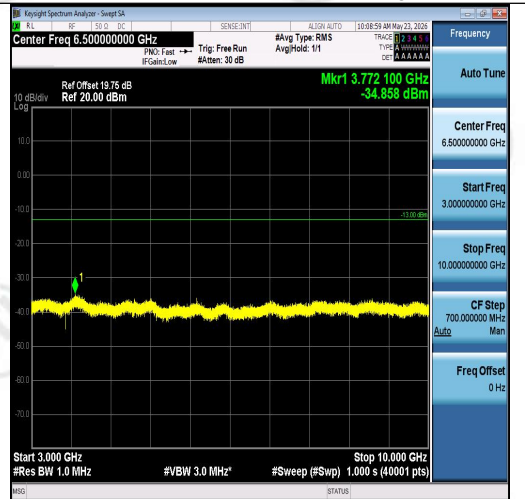
Band26(814-824)-5MHz-16QAM-26715-25RB#0 -3000~10000-PASS
