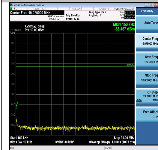
Band26(814-824)-5MHz-16QAM-26715-25RB#0 -0.15~30-PASS
