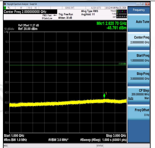
Band26(814-824)-5MHz-16QAM-26740-1RB#24 -1000~3000-PASS
