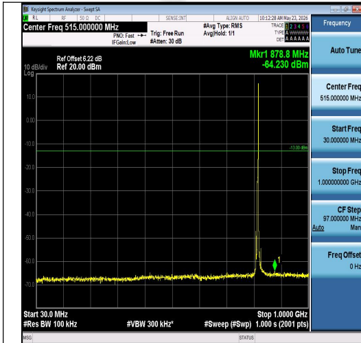
Band26(814-824)-5MHz-16QAM-26740-1RB#24 -30~1000-PASS
