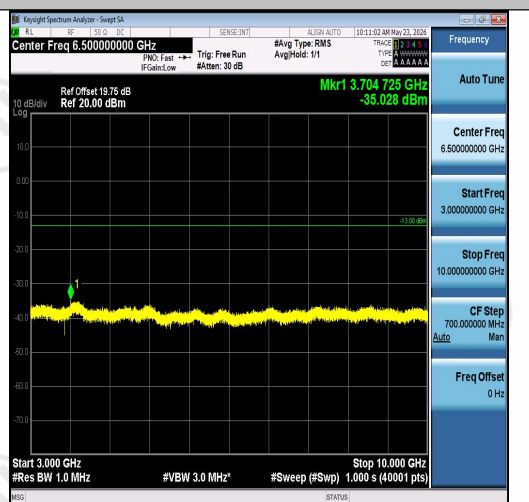
Band26(814-824)-5MHz-16QAM-26740-1RB#0-3000~10000-PASS
