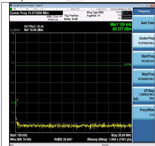
Band26(814-824)-5MHz-16QAM-26740-1RB#0-0.15~30-PASS
