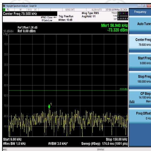
Band7-5MHz-QPSK-20775-1RB#24-0.009~0.15-
