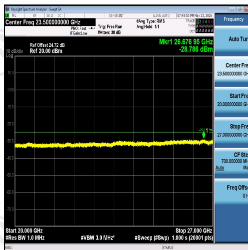
Band7-5MHz-QPSK-20775-1RB#0-20000~2700 0-PASS
