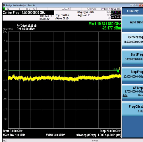
Band7-5MHz-QPSK-20775-1RB#0-3000~20000- PASS
