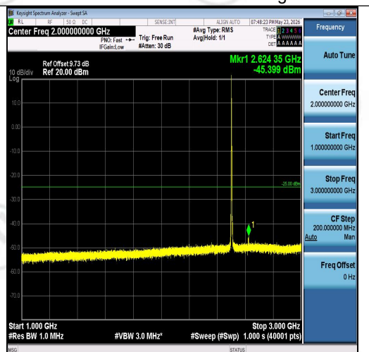
Band7-5MHz-QPSK-20775-1RB#0-1000~3000-P ASS
