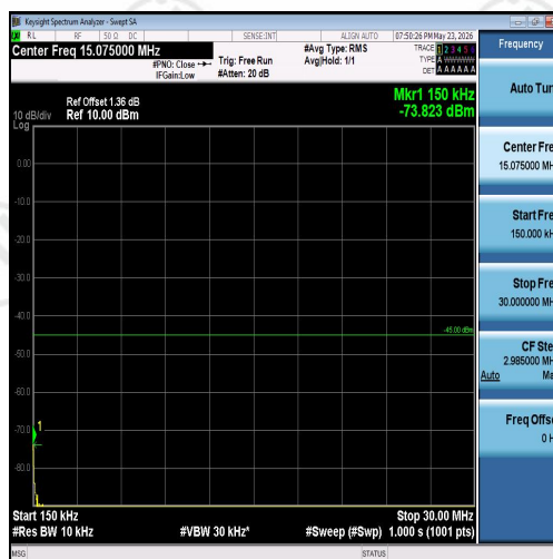
Band7-5MHz-QPSK-20775-1RB#24-0.15~30-PA
