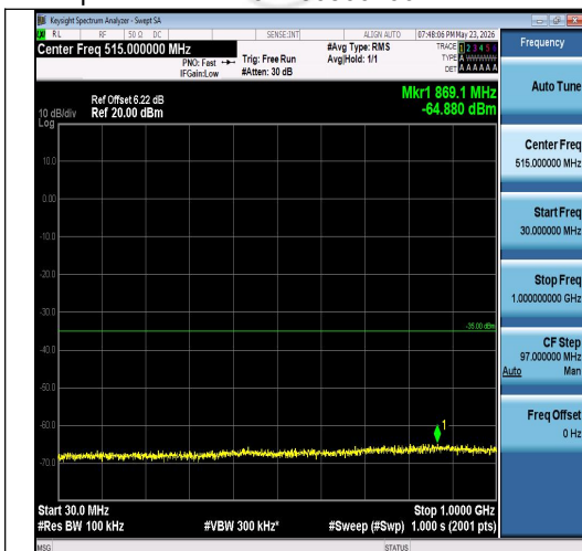
Band7-5MHz-QPSK-20775-1RB#0-30~1000-PA SS
