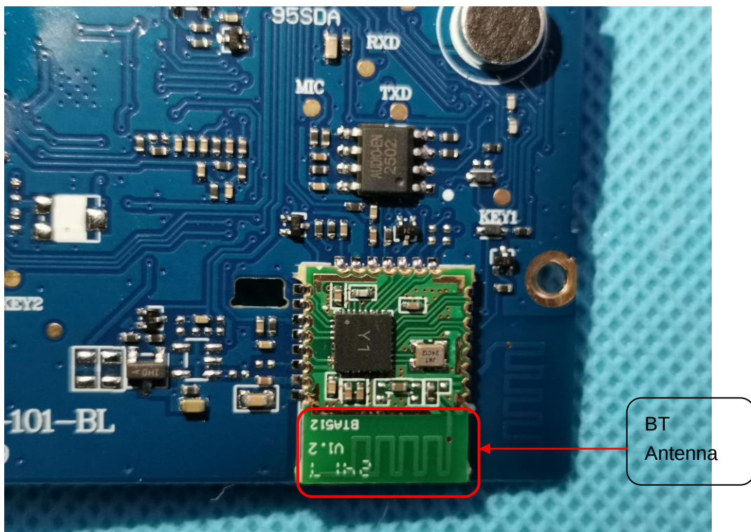
Internal View-12 of EUT
