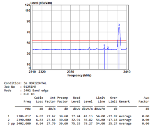
BLE_1M_TX_CH_00_Horizontal-AVG
