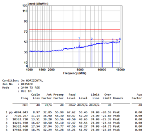
BLE_1M_TX_CH_19_Horizontal
