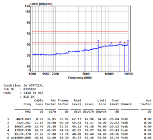
BLE_1M_TX_CH_19_Vertical
