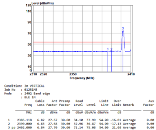
BLE_1M_TX_CH_00_Vertical-AVG
