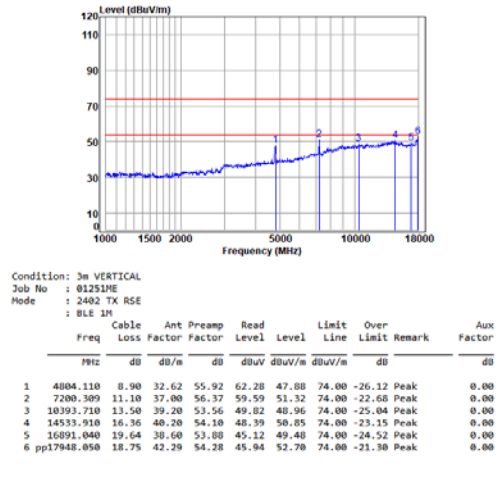
BLE_1M_TX_CH_00_Vertical
