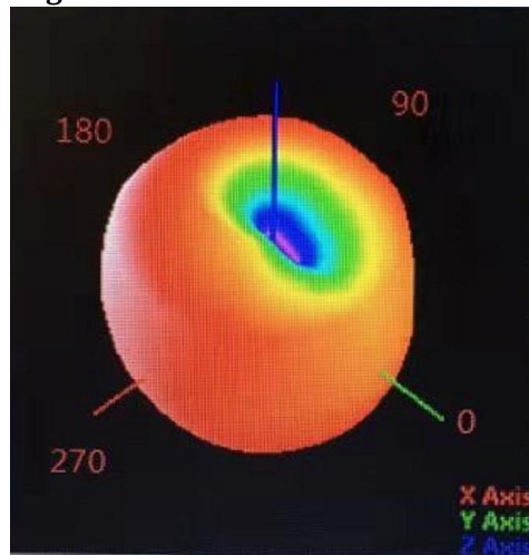
Figure 3. Radiation Pattern@2402MHz when DUT at \phi=0^\circ , \theta=0^\circ
