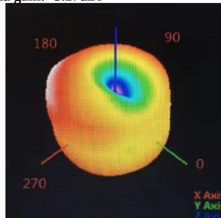
Figure 5. Radiation Pattern@2480MHz when DUT at \phi=0^\circ , \theta=0^\circ
