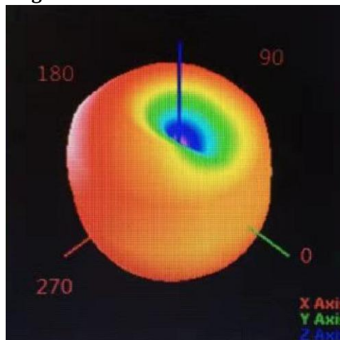
Figure 4. Radiation Pattern@2441MHz when DUT at \phi=0^\circ , \theta=0^\circ
