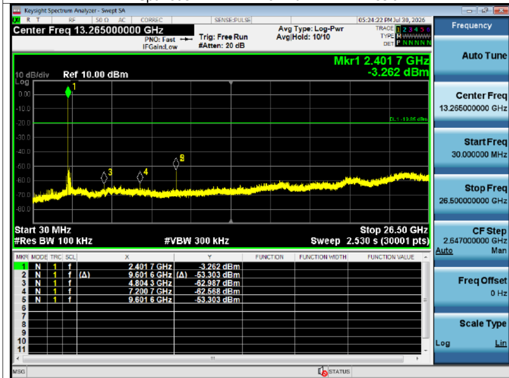
Tx. Spurious NVNT 2-DH5 2402MHz Emission
