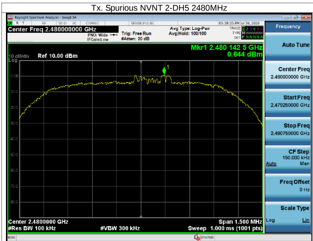
Tx. Spurious NVNT 2-DH5 2480MHz Emission
