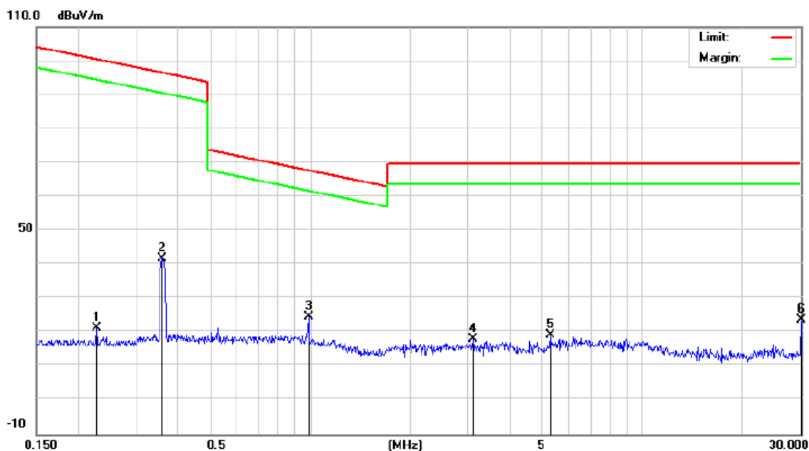
Test graph and data for Electric Field strength between 150kHz-30MHz
