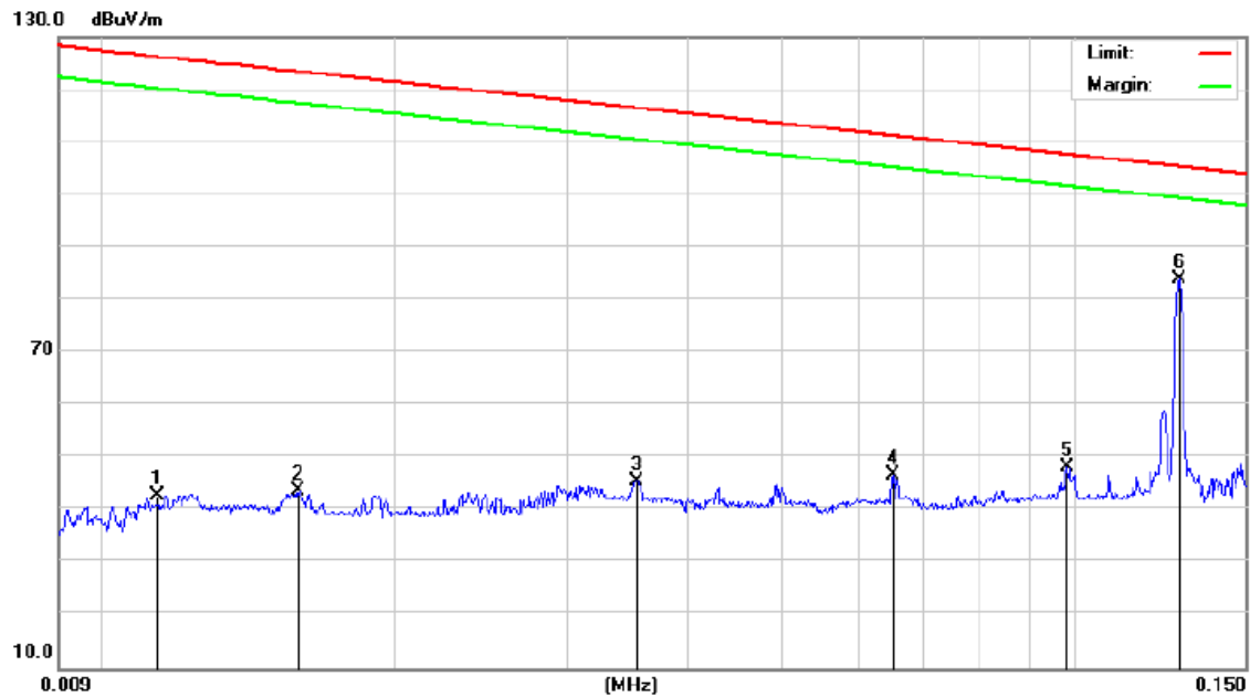
Test graph and data for Electric Field strength between 9kHz-150kHz
