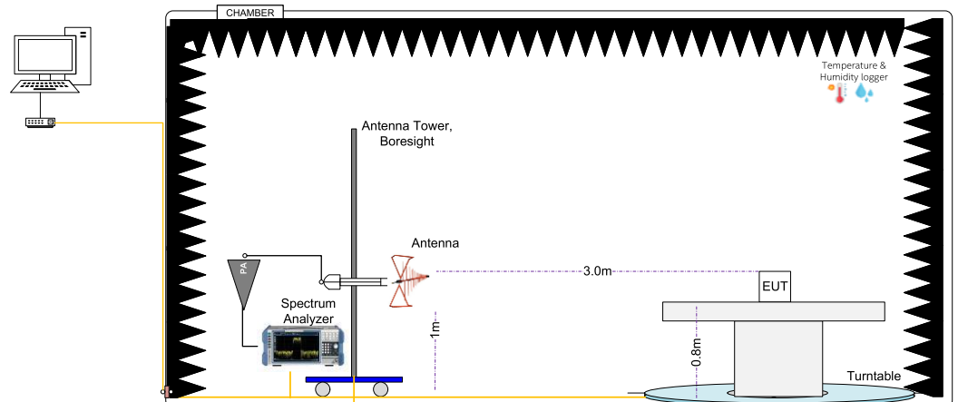
Radiated Setup 30MHz - 1GHz (Transmitter tests)
