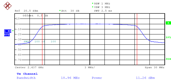
Mode: TX 11ax HE20 channel 6
