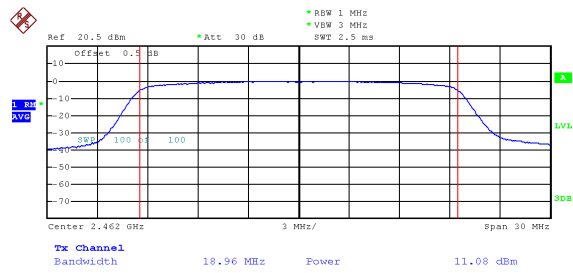
Mode: TX 11ax HE20 channel 11
