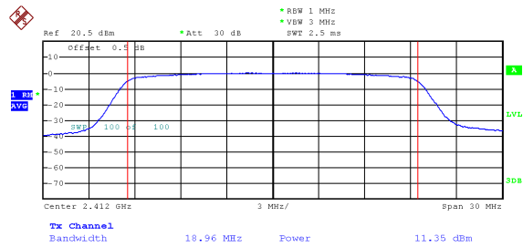
Mode: TX 11ax HE20 channel 1
