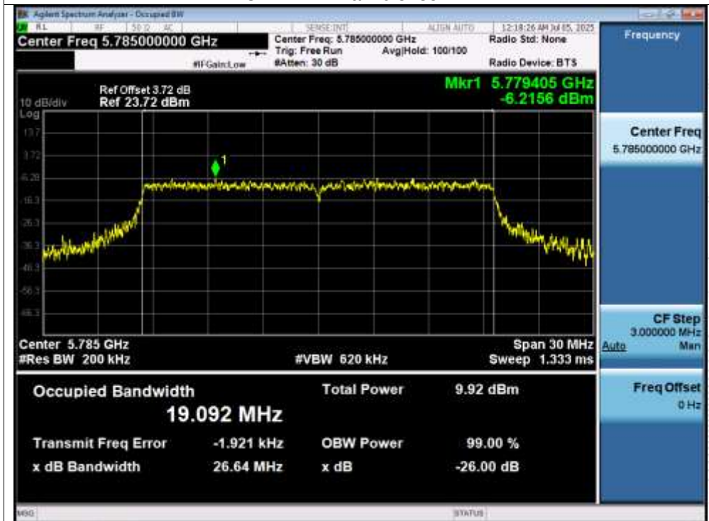
OBW NVNT ax20 5785MHz
