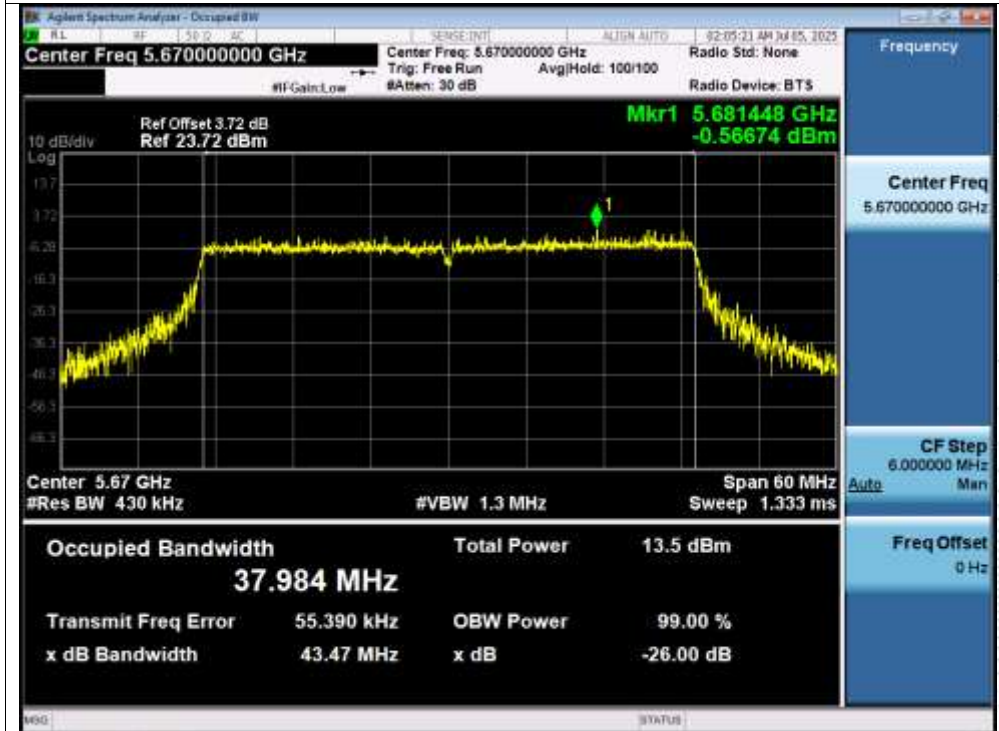
-26dB Bandwidth NVNT ax40 5670MHz
