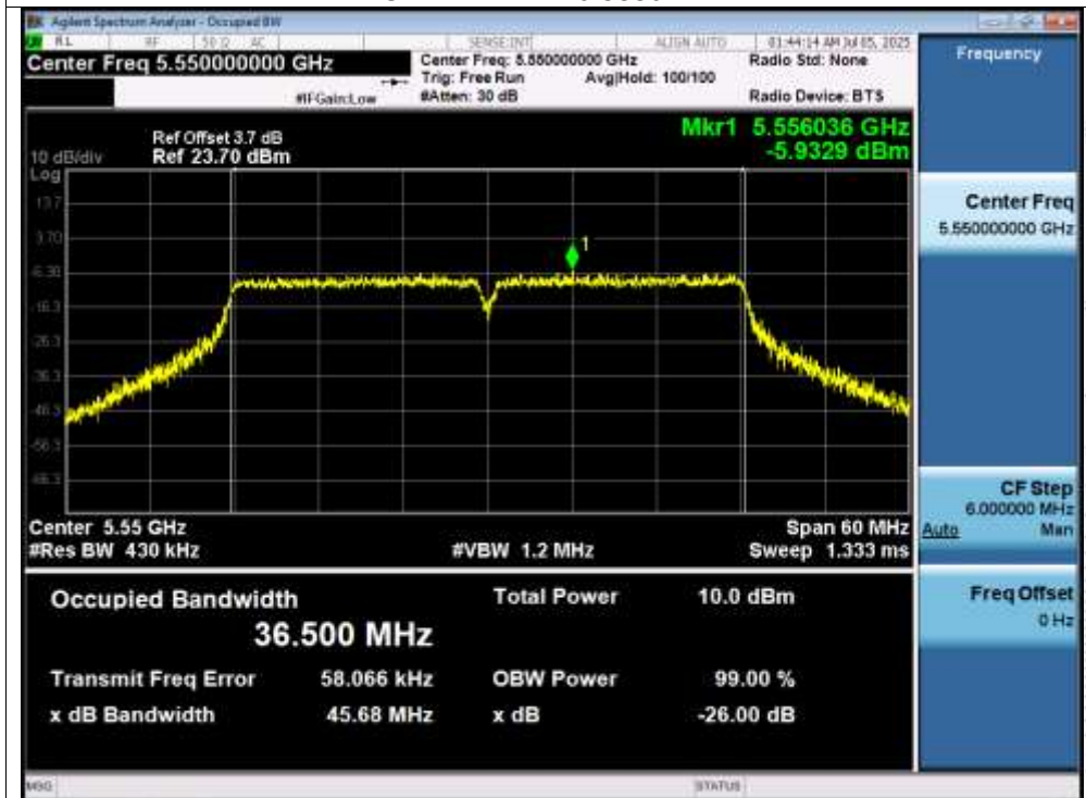
OBW NVNT n40 5550MHz
