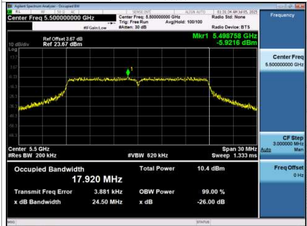
OBW NVNT n20 5500MHz
