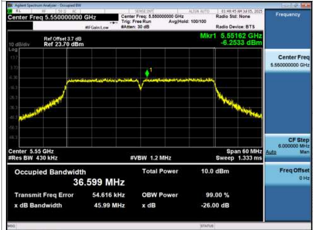
OBW NVNT ac40 5550MHz
