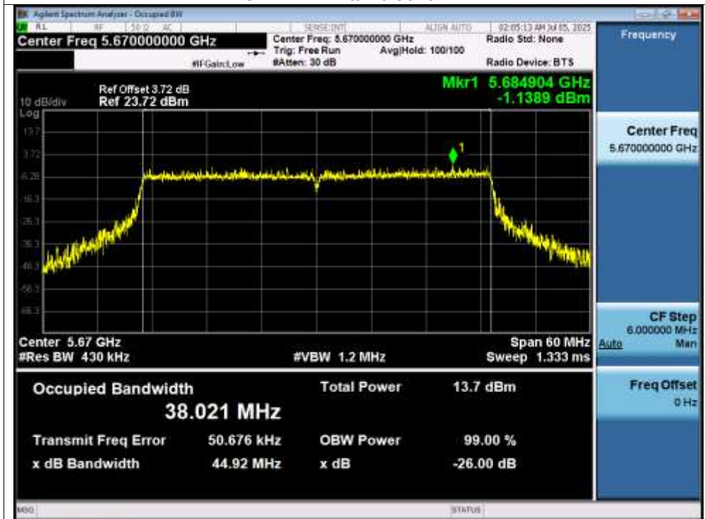
OBW NVNT ax40 5670MHz
