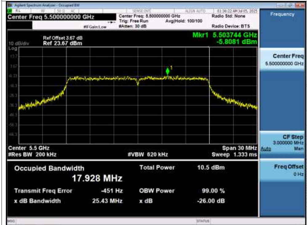
-26dB Bandwidth NVNT ac20 5500MHz
