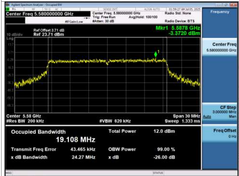
OBW NVNT ax20 5580MHz
