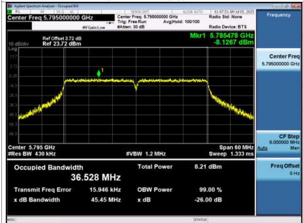
OBW NVNT n40 5795MHz
