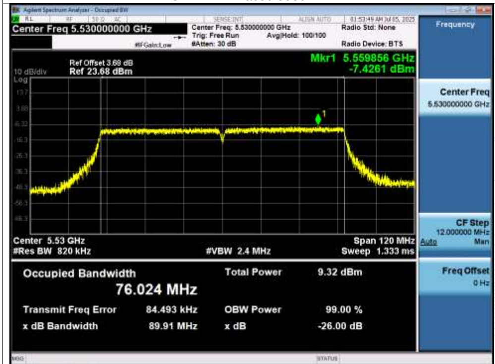
OBW NVNT ac80 5530MHz
