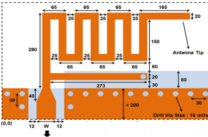
Antenna Photo &amp; Length (mm)
