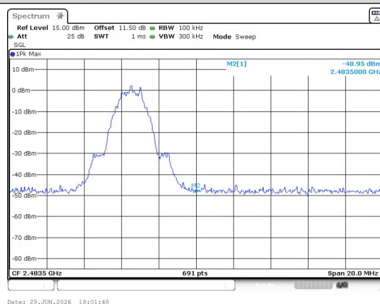
Out Of Band Emission BLE 2M_Channel 39
