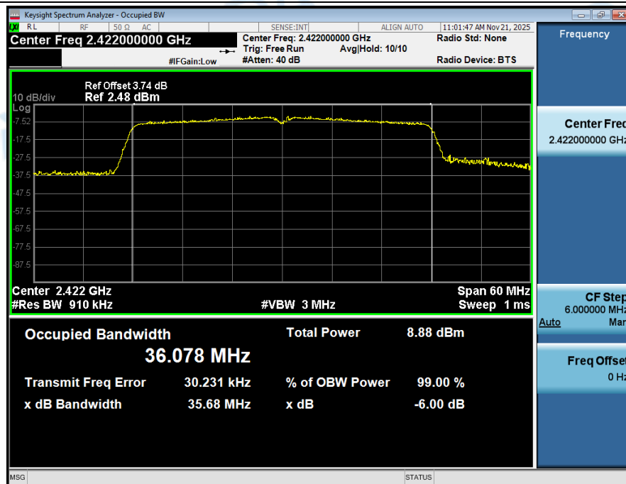
-6dB_Bandwidth_NVNT_ANT1_802_11n(HT40)_2422
