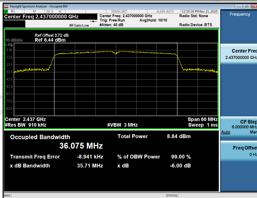
-6dB_Bandwidth_NVNT_ANT1_802_11n(HT40)_2437
