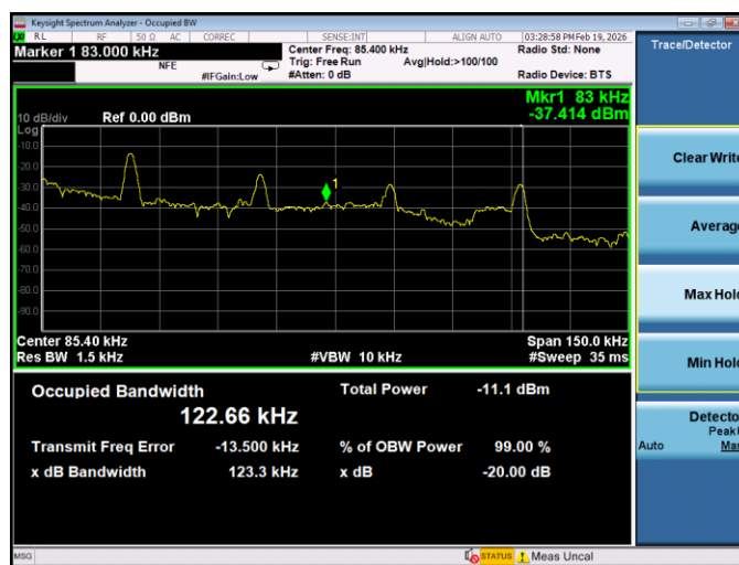
Figure 1-1 WPT Occupied Bandwidth
