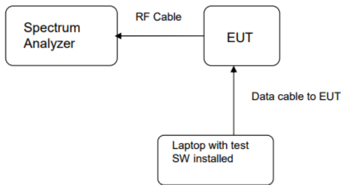
Diagram of Measurement Configuration for Conduction Test (Floor-standing)
