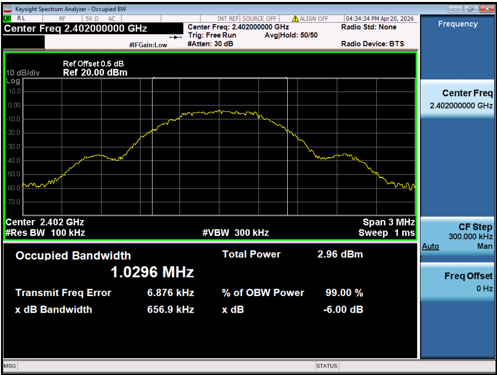
Figure 4: 6dB Bandwidth, 2402MHz
