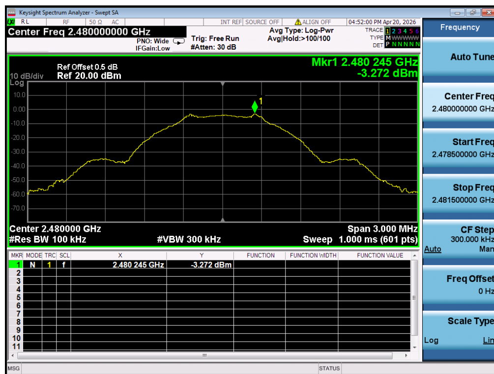
Figure 12: Conducted Spurious Emission & Authorized-band band-edge, 2480MHz, BLE Carrier Level
