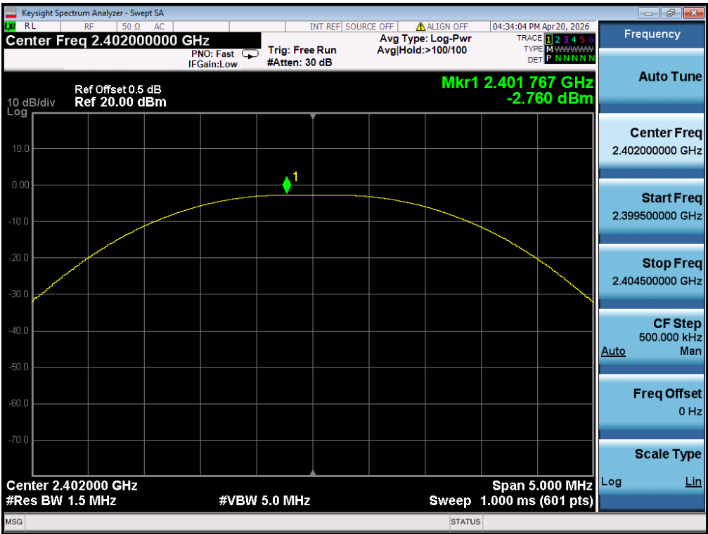
Figure 1: Peak Output Power, 2402MHz
