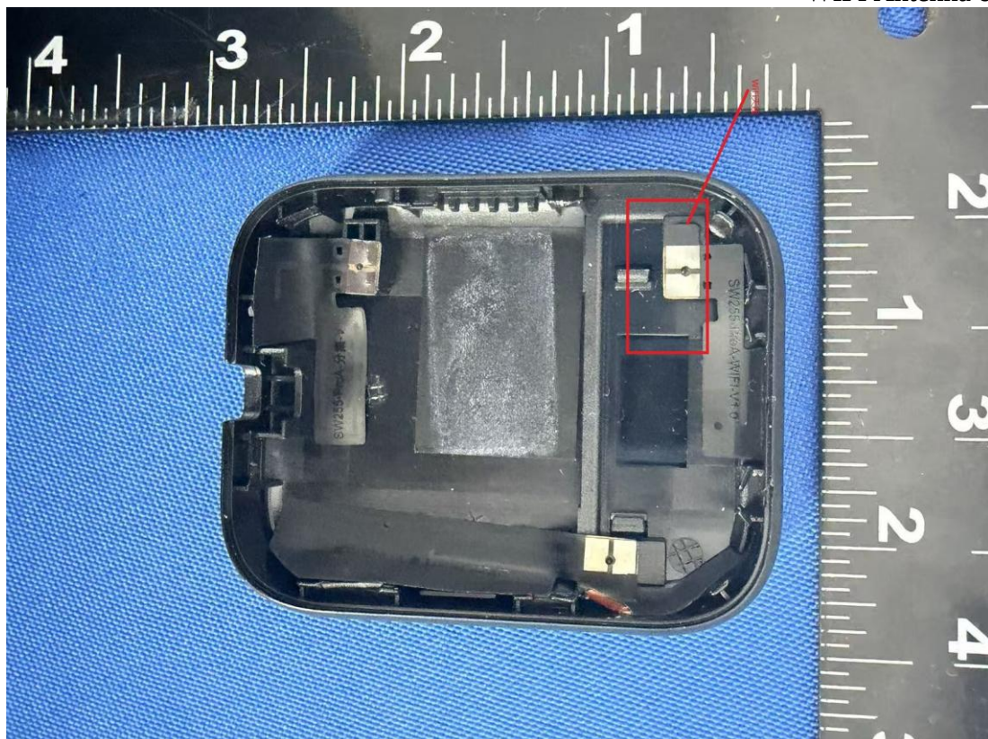
Figure 20 WIFI Antenna of the EUT
