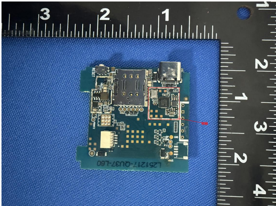
Figure 19 Module of the EUT
