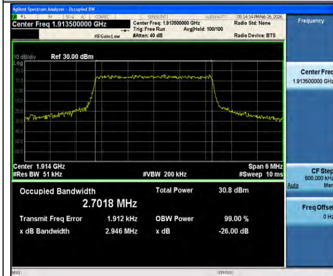
Band25-3MHz-QPSK-26675-15RB#0-PASS
