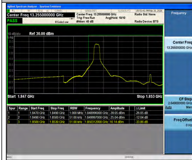
Band25-5MHz-QPSK-26065-1RB#0-PASS
