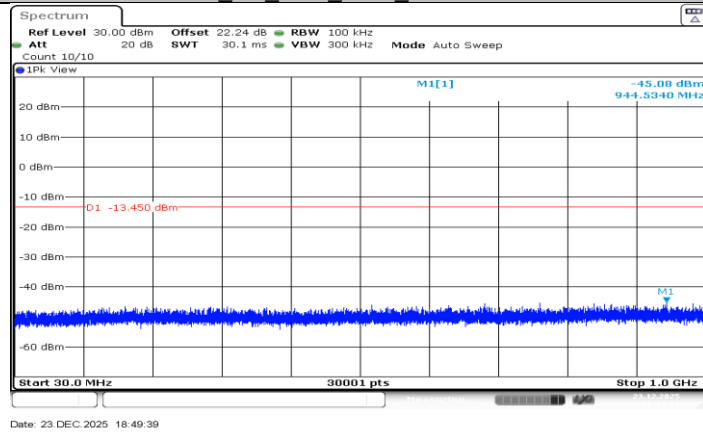
BLE_2M_Ant3_2402_30~1000
