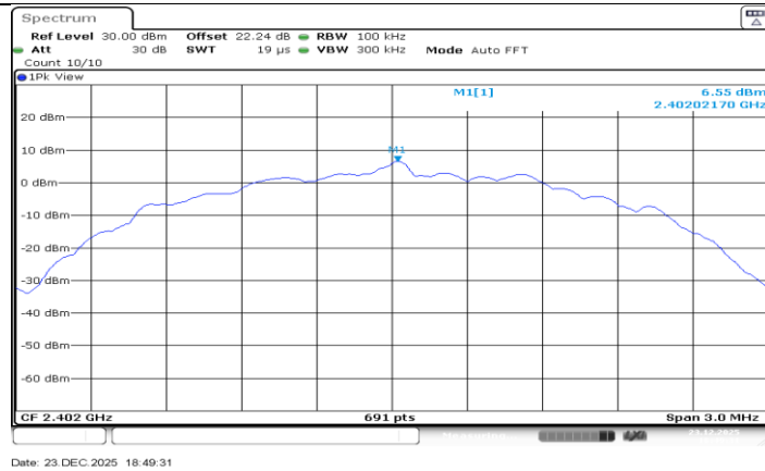
BLE_2M_Ant3_2402_0~Reference
