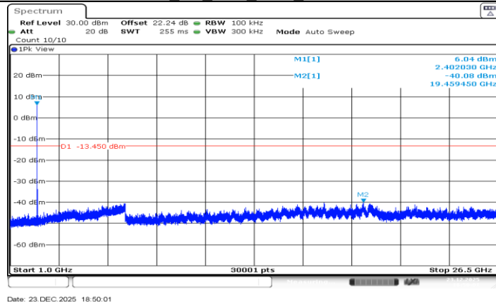
BLE_2M_Ant3_2402_1000~26500
