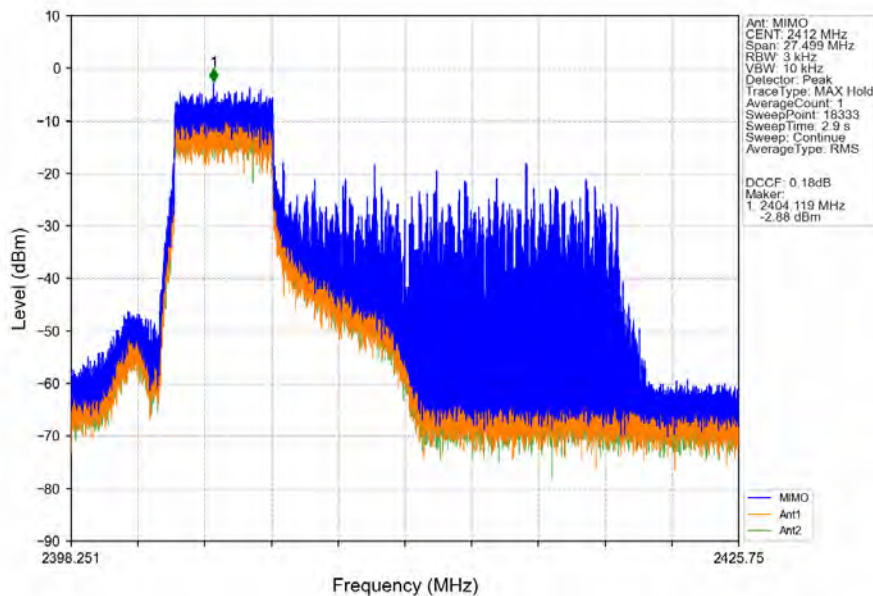
802.11ax(HEW20)_LCH_2412MHz_RU52_Left_MIMO_NTNV
