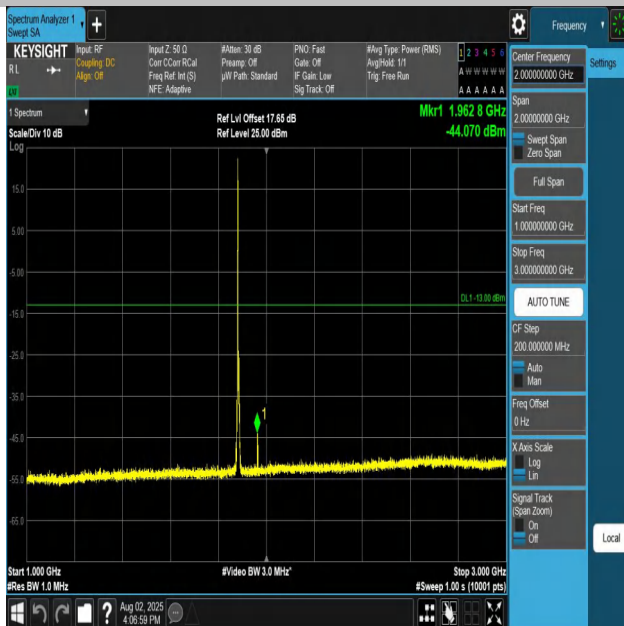
Band25-5MHz-QPSK-26365-1RB#0-1000~3000-PASS
