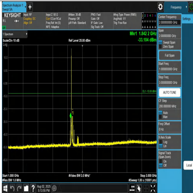
Band25-20MHz-QPSK-26140-1RB#0-1000~3000-PASS
