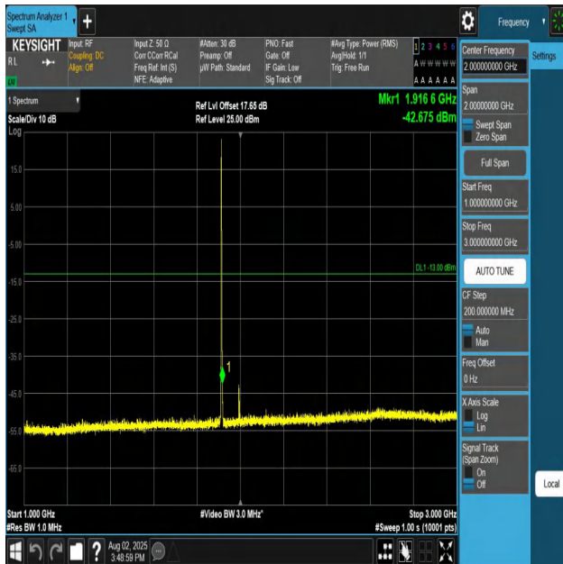
Band25-3MHz-QPSK-26675-1RB#0-1000~3000-PASS
