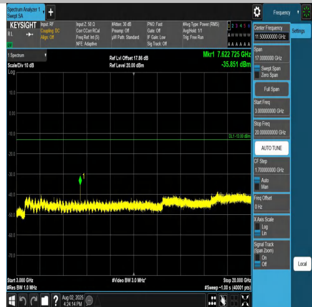
Band25-10MHz-QPSK-26640-1RB#0-3000~20000-PASS
