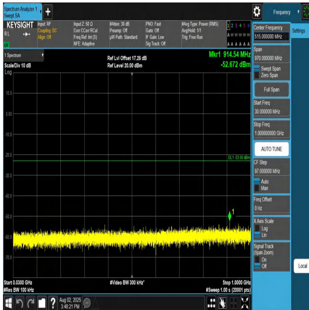
Band25-3MHz-QPSK-26365-1RB#0-30~1000-PASS
