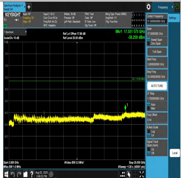
Band25-3MHz-QPSK-26055-1RB#0-3000~20000-PASS
