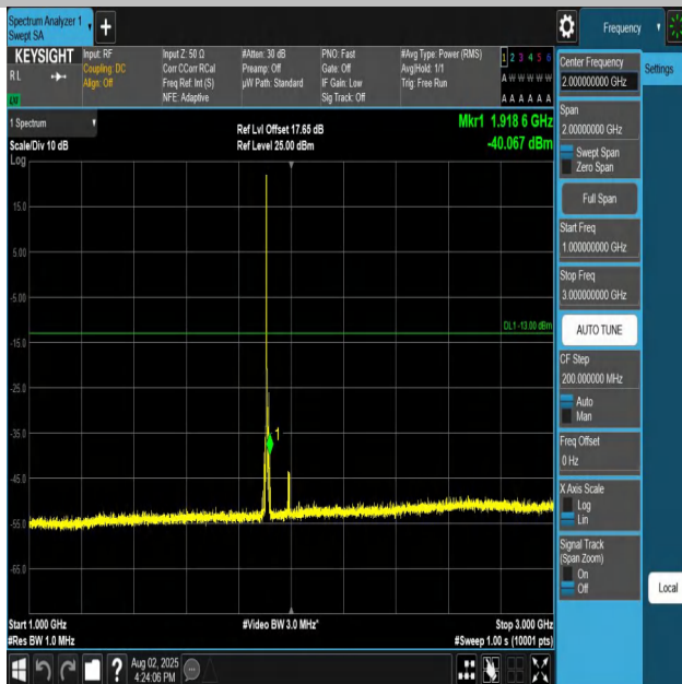
Band25-10MHz-QPSK-26640-1RB#0-1000~3000-PASS
