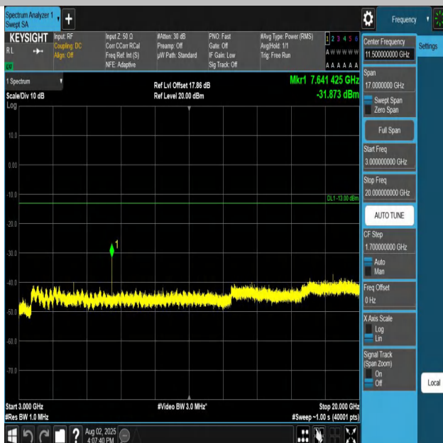
Band25-5MHz-QPSK-26665-1RB#0-3000~20000-PASS
