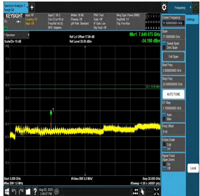
Band25-3MHz-QPSK-26675-1RB#0-3000~20000-PASS
