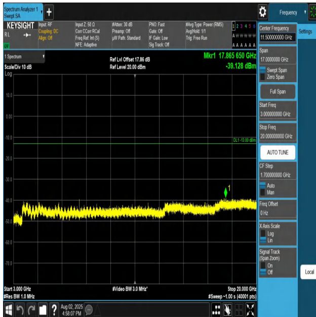
Band25-15MHz-QPSK-26615-1RB#0-3000~20000-PASS
