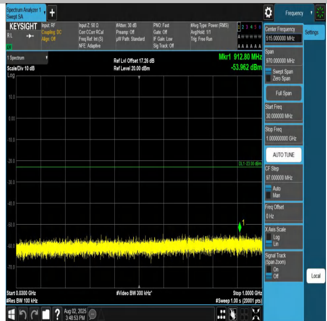
Band25-3MHz-QPSK-26675-1RB#0-30~1000-PASS
