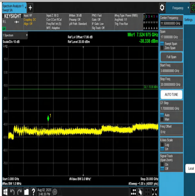
Band25-3MHz-QPSK-26365-1RB#0-3000~20000-PASS
