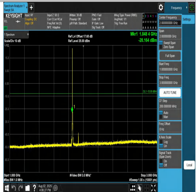
Band25-5MHz-QPSK-26065-1RB#0-1000~3000-PASS
