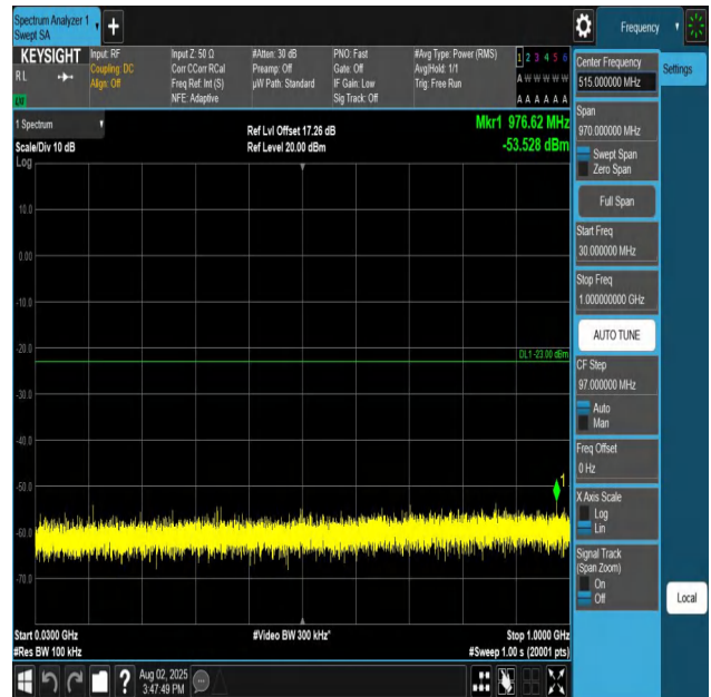
Band25-3MHz-QPSK-26055-1RB#0-30~1000-PASS
