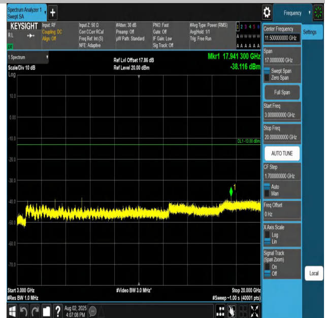
Band25-5MHz-QPSK-26365-1RB#0-3000~20000-PASS
