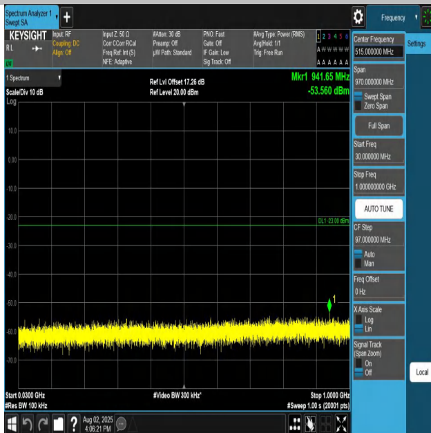
Band25-5MHz-QPSK-26065-1RB#0-30~1000-PASS
