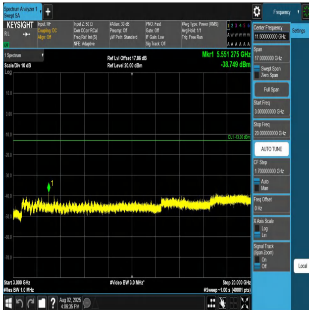
Band25-5MHz-QPSK-26065-1RB#0-3000~20000-PASS
