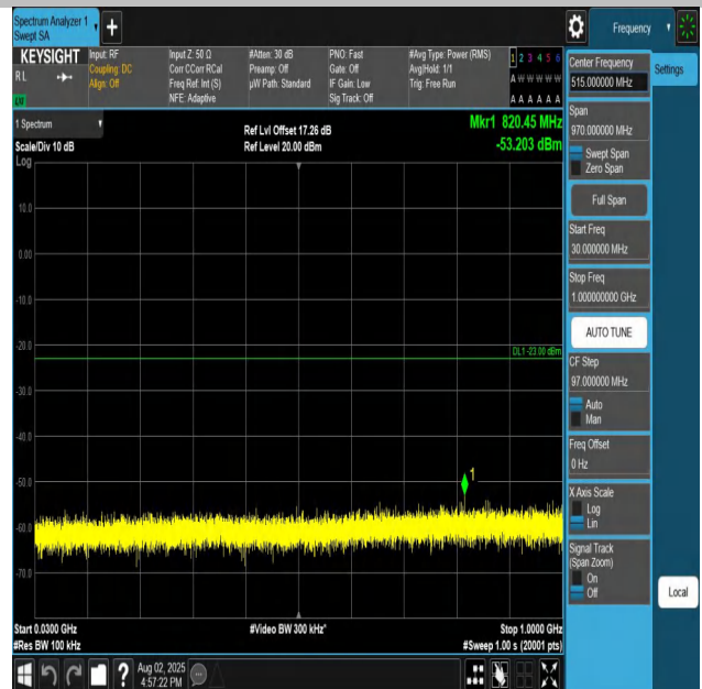
Band25-15MHz-QPSK-26365-1RB#0-30~1000-PASS
