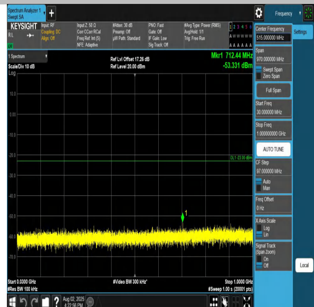
Band25-10MHz-QPSK-26090-1RB#0-30~1000-PASS
