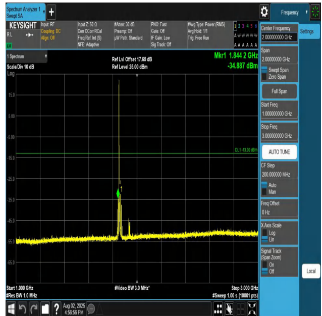
Band25-15MHz-QPSK-26115-1RB#0-1000~3000-PASS
