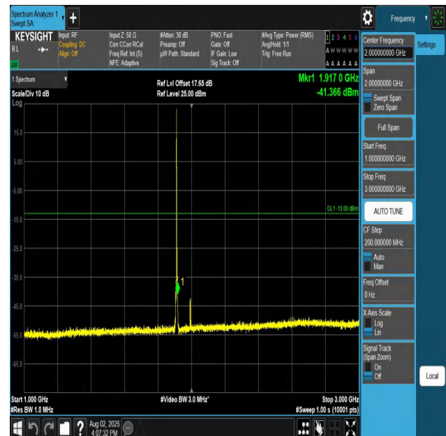
Band25-5MHz-QPSK-26665-1RB#0-1000~3000-PASS
