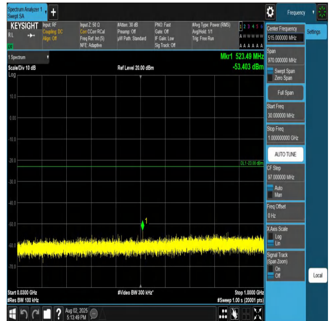
Band25-20MHz-QPSK-26140-1RB#0-30~1000-PASS
