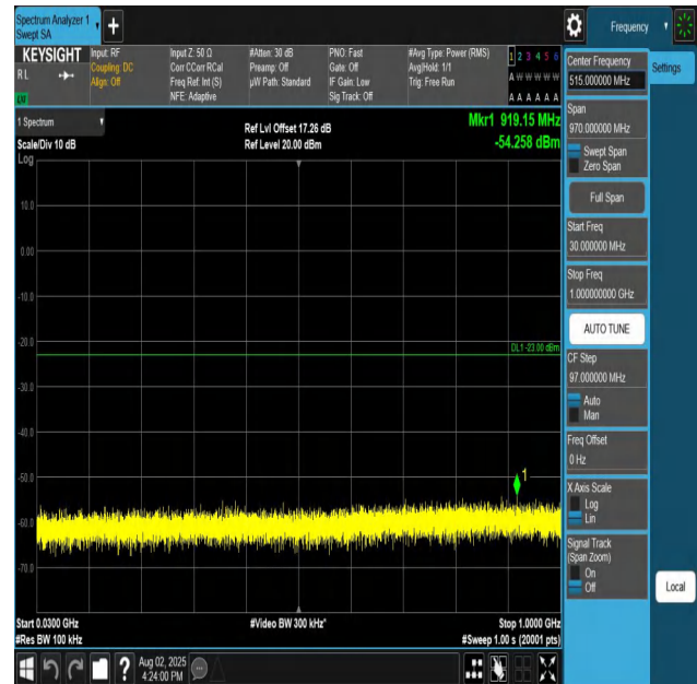
Band25-10MHz-QPSK-26640-1RB#0-30~1000-PASS
