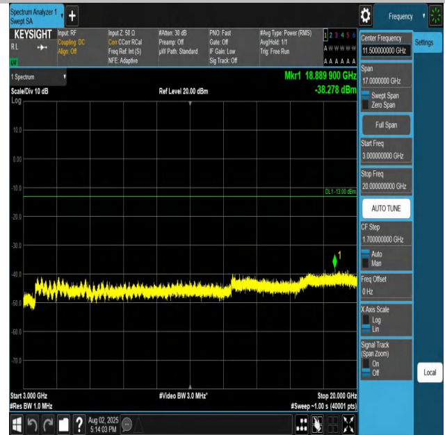
Band25-20MHz-QPSK-26140-1RB#0-3000~20000-PASS
