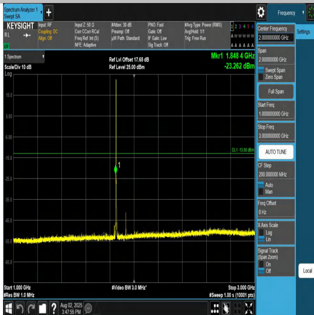
Band25-3MHz-QPSK-26055-1RB#0-1000~3000-PASS
