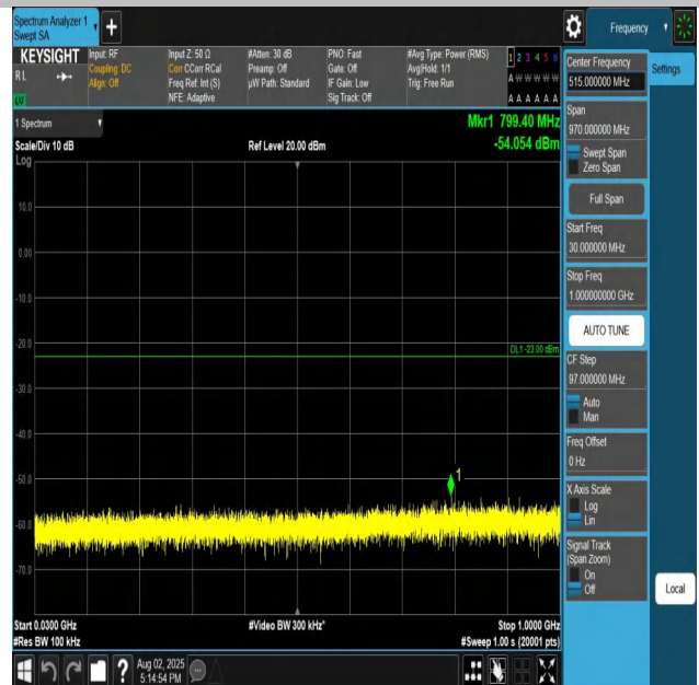
Band25-20MHz-QPSK-26590-1RB#0-30~1000-PASS
