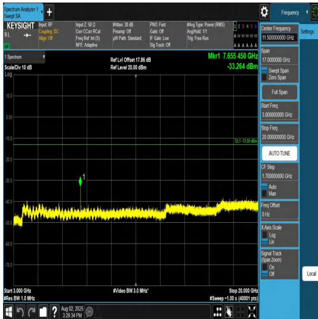
Band25-1.4MHz-QPSK-26683-1RB#0-3000~20000-PASS
