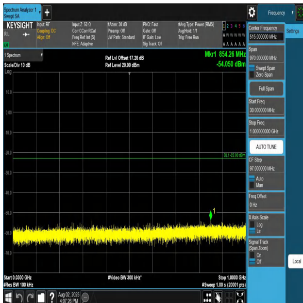
Band25-5MHz-QPSK-26665-1RB#0-30~1000-PASS
