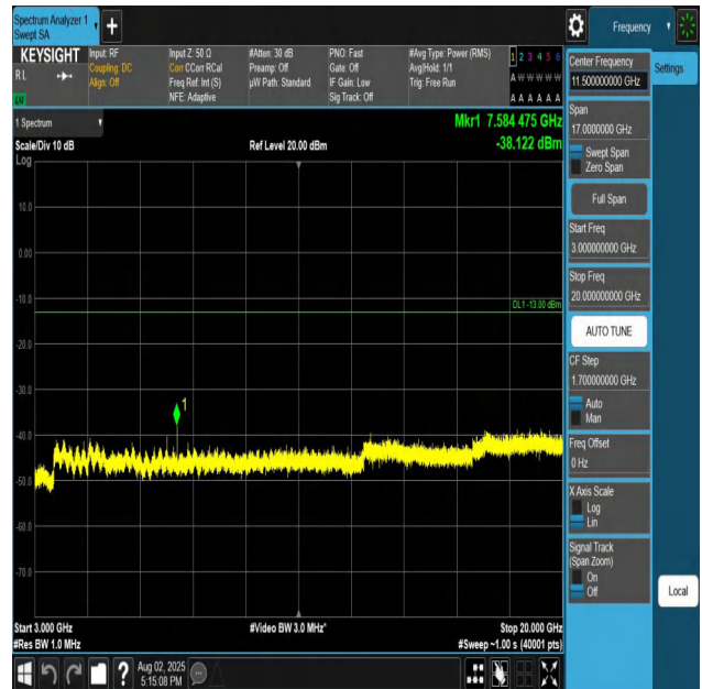
Band25-20MHz-QPSK-26590-1RB#0-3000~20000-PASS
