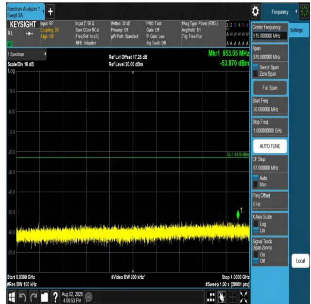
Band25-5MHz-QPSK-26365-1RB#0-30~1000-PASS
