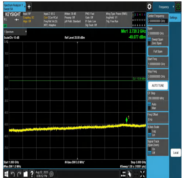
Band26(824-849)-15MHz-QPSK-26865-1RB#0-1000~300 0-PASS
