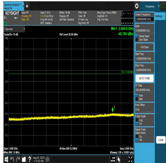
Band26(824-849)-5MHz-QPSK-27015-1RB#0-1000~3000-P PASS
