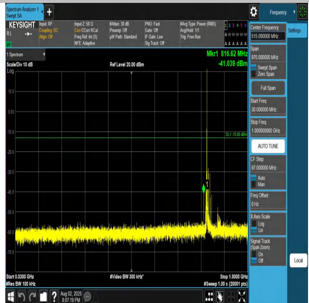
Band26(824-849)-15MHz-QPSK-26915-1RB#0-30~1000-P ASS
