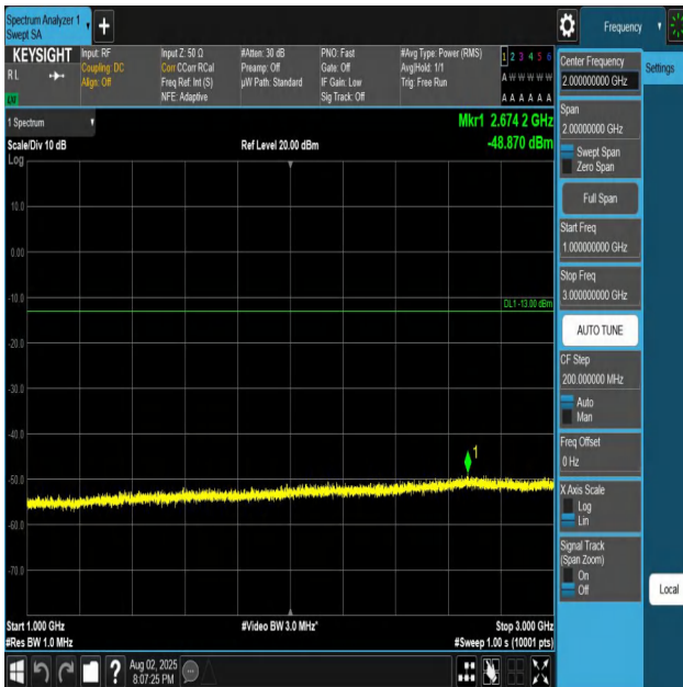
Band26(824-849)-15MHz-QPSK-26915-1RB#0-1000~300 0-PASS
