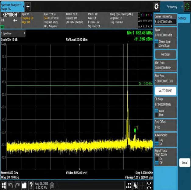
Band26(824-849)-10MHz-QPSK-26915-1RB#0-30~1000-P ASS
