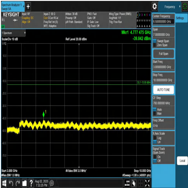
Band26(824-849)-10MHz-QPSK-26840-1RB#0-3000~100 00-PASS
