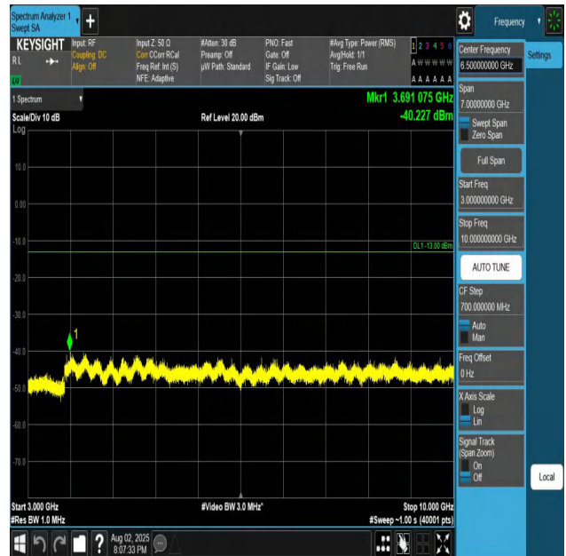
Band26(824-849)-15MHz-QPSK-26915-1RB#0-3000~100 00-PASS
