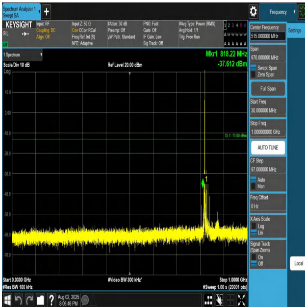
Band26(824-849)-15MHz-QPSK-26865-1RB#0-30~1000-P ASS
