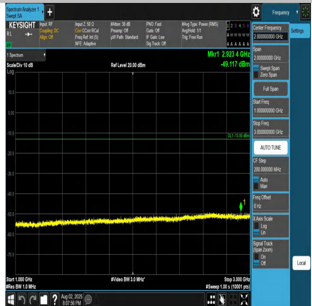
Band26(824-849)-15MHz-QPSK-26965-1RB#0-1000~300 0-PASS
