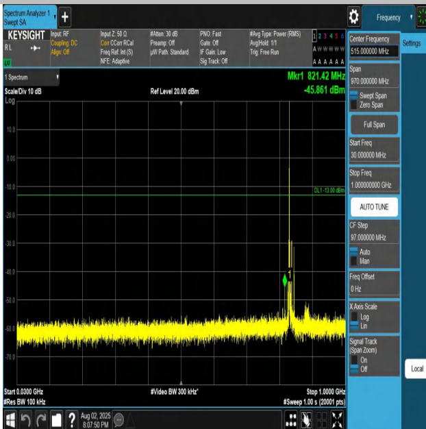
Band26(824-849)-15MHz-QPSK-26965-1RB#0-30~1000-P ASS
