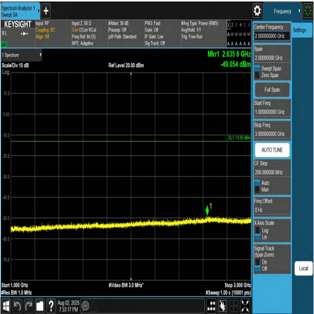
Band26(824-849)-10MHz-QPSK-26840-1RB#0-1000~300 0-PASS
