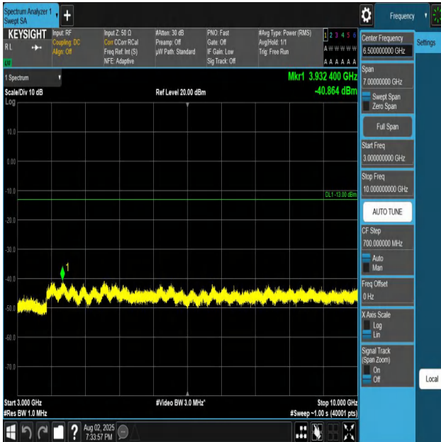
Band26(824-849)-10MHz-QPSK-26915-1RB#0-3000~100 00-PASS
