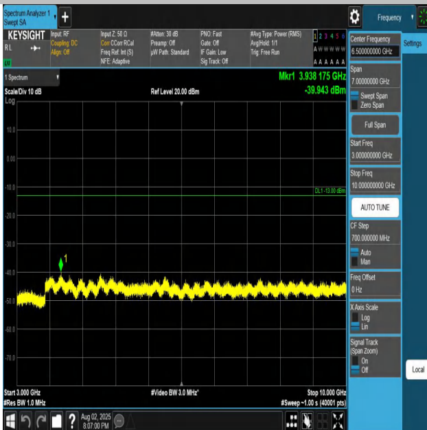
Band26(824-849)-15MHz-QPSK-26865-1RB#0-3000~100 00-PASS
