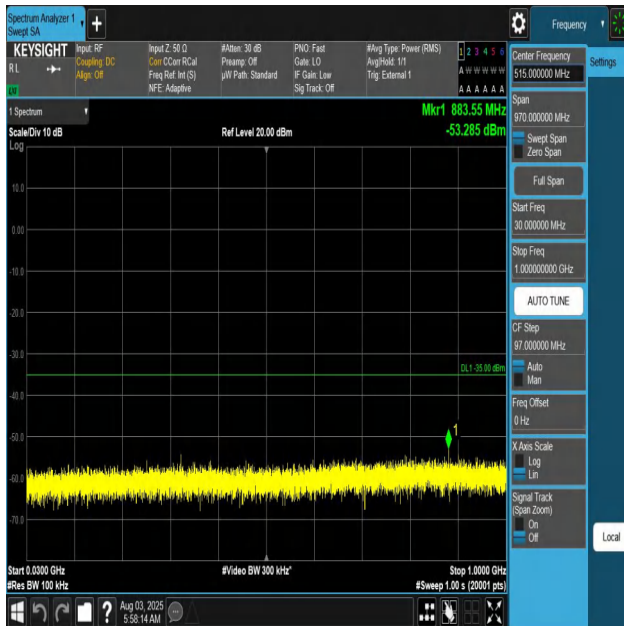
Band41-20MHz-QPSK-40620-1RB#0-30~1000-PASS
