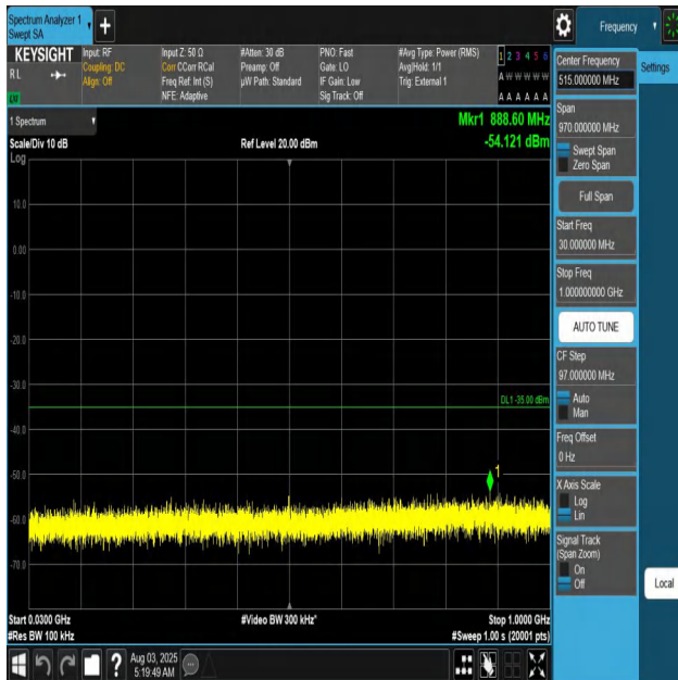
Band41-15MHz-QPSK-39725-1RB#0-30~1000-PASS
