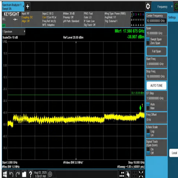
Band41-20MHz-QPSK-40620-1RB#0-3000~18000-PASS
