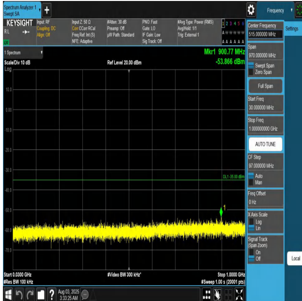
Band41-5MHz-QPSK-39675-1RB#0-30~1000-PASS
