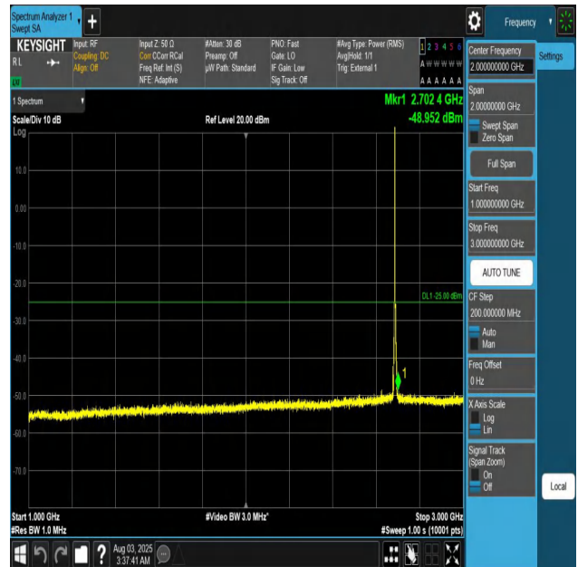
Band41-5MHz-QPSK-41565-1RB#0-1000~3000-PASS
