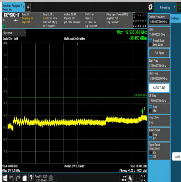
Band41-15MHz-QPSK-39725-1RB#0-3000~18000-PASS
