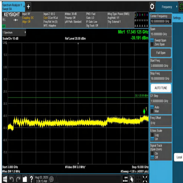
Band41-5MHz-QPSK-40620-1RB#0-3000~18000-PASS
