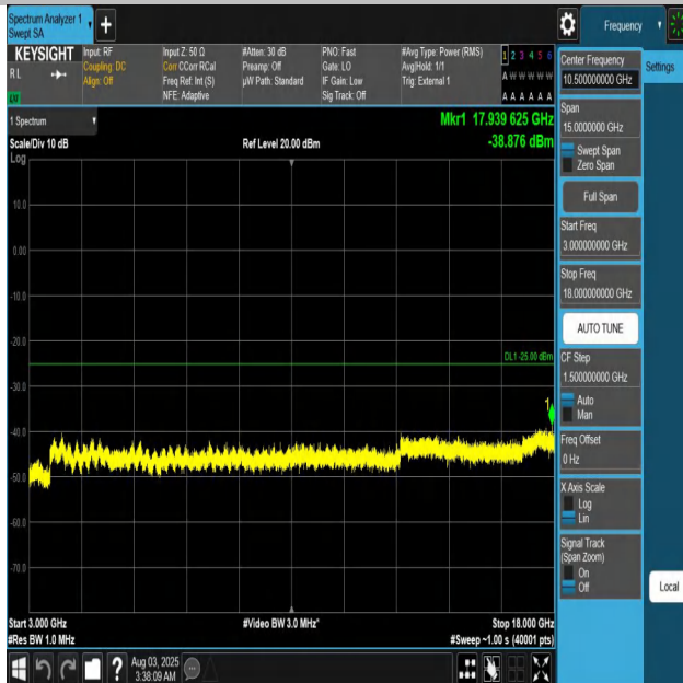
Band41-5MHz-QPSK-41565-1RB#0-3000~18000-PASS
