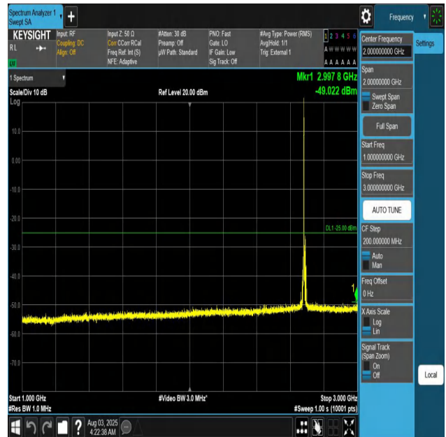
Band41-10MHz-QPSK-41540-1RB#0-1000~3000-PASS
