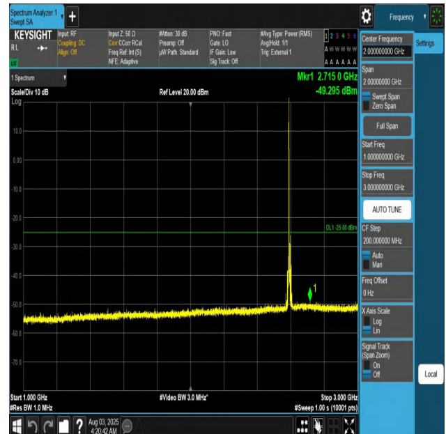
Band41-10MHz-QPSK-40620-1RB#0-1000~3000-PASS
