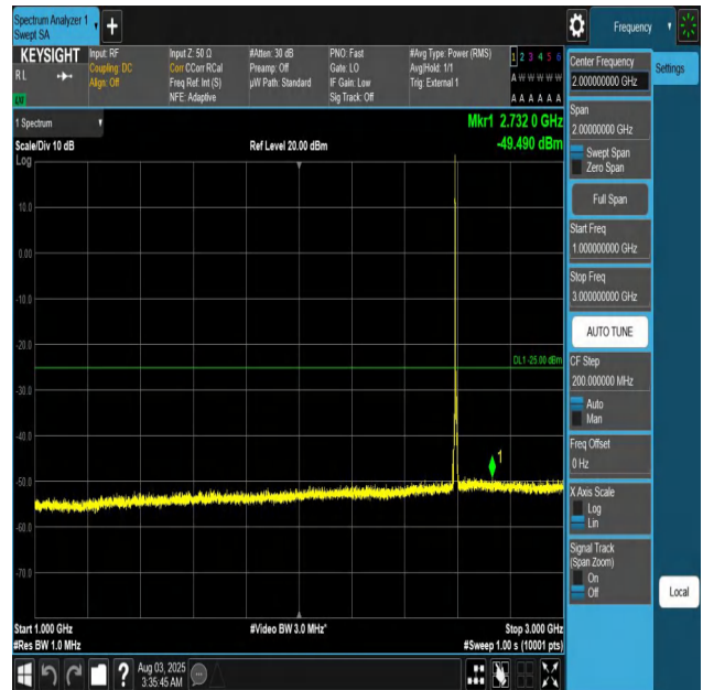
Band41-5MHz-QPSK-40620-1RB#0-1000~3000-PASS
