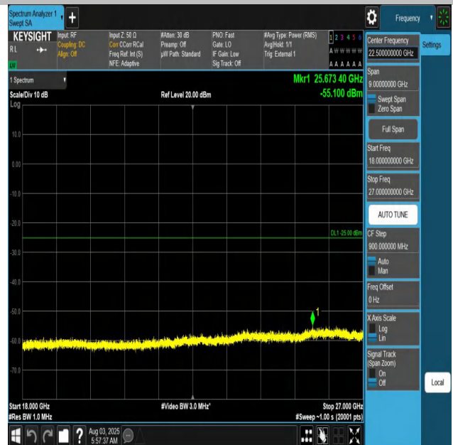
Band41-20MHz-QPSK-39750-1RB#0-18000~27000-PASS
