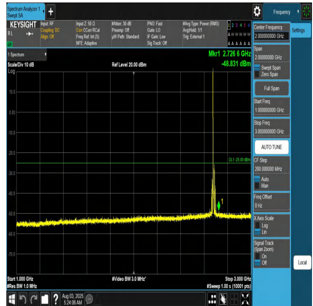
Band41-15MHz-QPSK-41515-1RB#0-1000~3000-PASS
