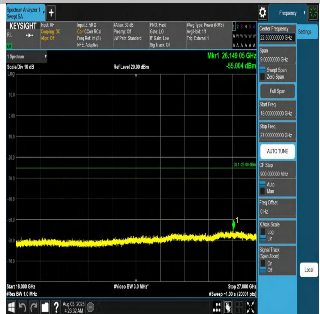
Band41-10MHz-QPSK-41540-1RB#0-18000~27000-PASS
