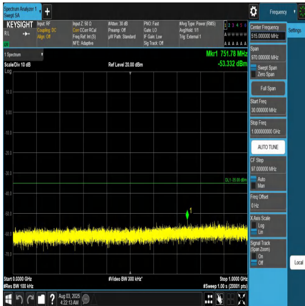
Band41-10MHz-QPSK-41540-1RB#0-30~1000-PASS
