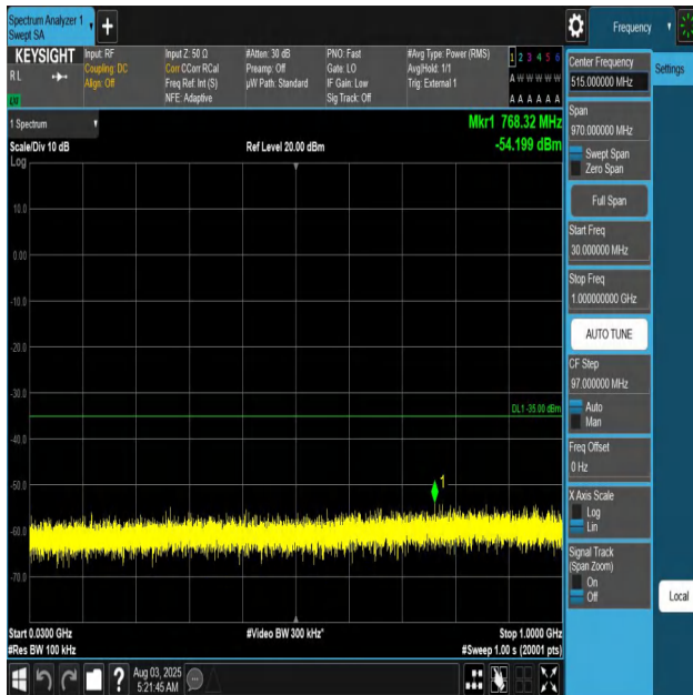
Band41-15MHz-QPSK-40620-1RB#0-30~1000-PASS
