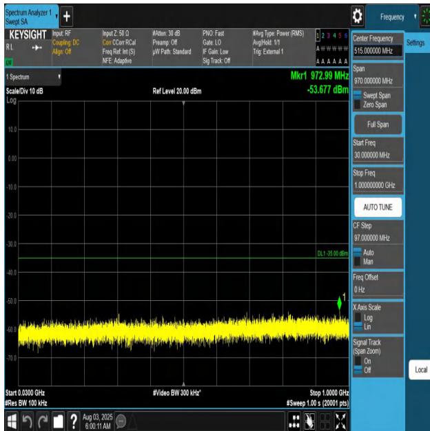
Band41-20MHz-QPSK-41490-1RB#0-30~1000-PASS
