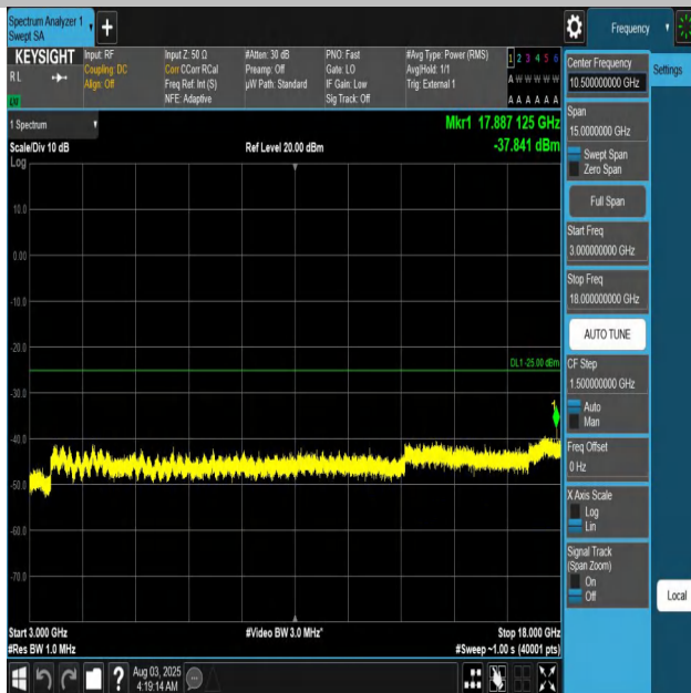
Band41-10MHz-QPSK-39700-1RB#0-3000~18000-PASS
