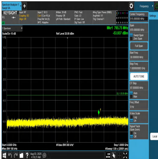
Band41-10MHz-QPSK-39700-1RB#0-30~1000-PASS
