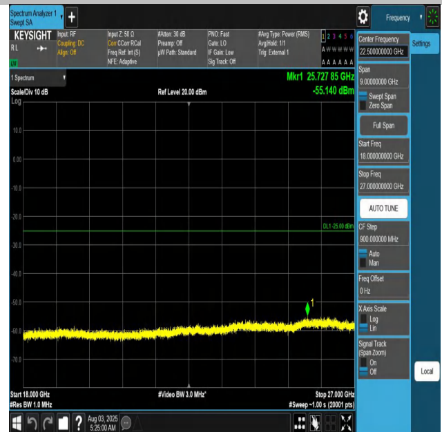
Band41-15MHz-QPSK-41515-1RB#0-18000~27000-PASS
