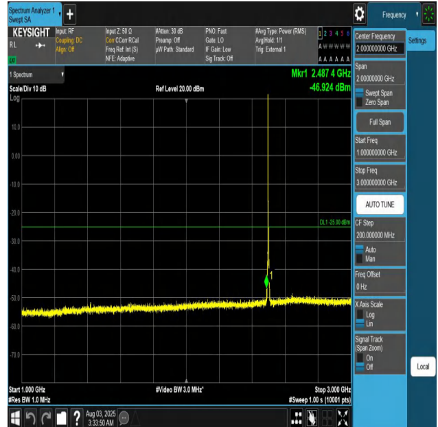
Band41-5MHz-QPSK-39675-1RB#0-1000~3000-PASS
