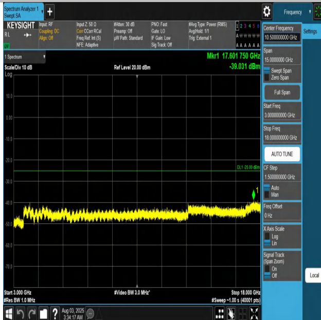
Band41-5MHz-QPSK-39675-1RB#0-3000~18000-PASS
