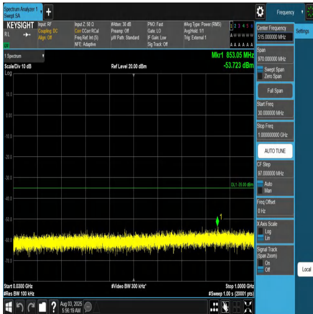
Band41-20MHz-QPSK-39750-1RB#0-30~1000-PASS
