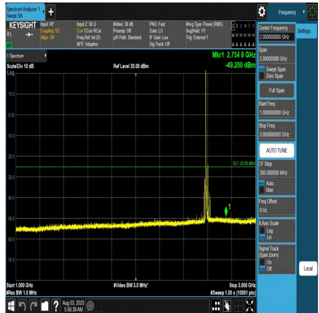
Band41-20MHz-QPSK-40620-1RB#0-1000~3000-PASS
