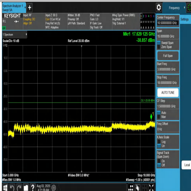
Band41-10MHz-QPSK-40620-1RB#0-3000~18000-PASS
