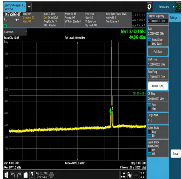
Band41-15MHz-QPSK-39725-1RB#0-1000~3000-PASS
