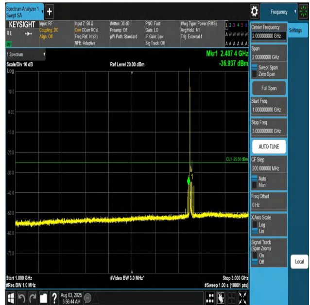
Band41-20MHz-QPSK-39750-1RB#0-1000~3000-PASS
