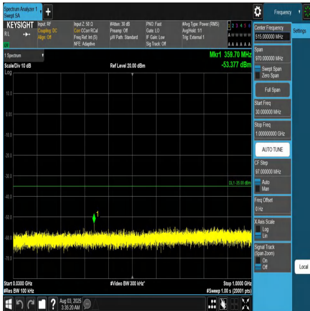
Band41-5MHz-QPSK-40620-1RB#0-30~1000-PASS
