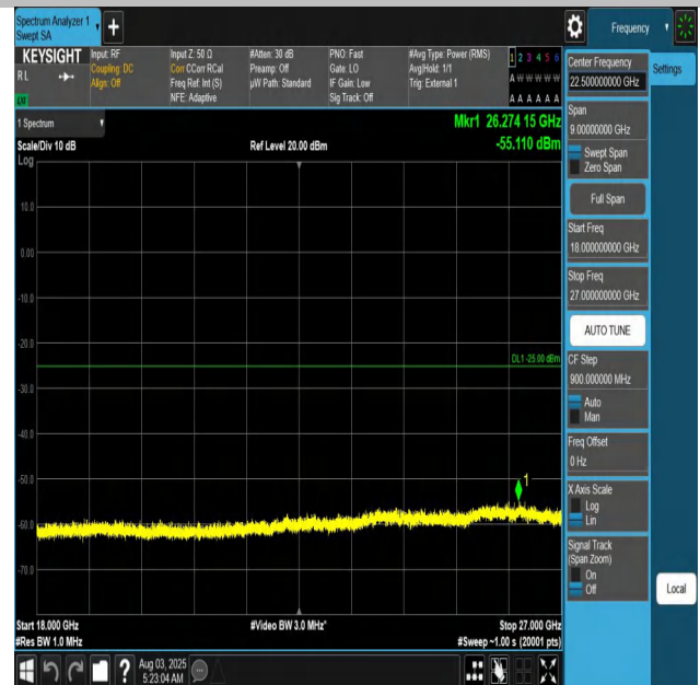
Band41-15MHz-QPSK-40620-1RB#0-18000~27000-PASS
