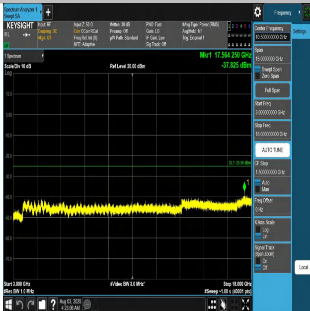
Band41-10MHz-QPSK-41540-1RB#0-3000~18000-PASS
