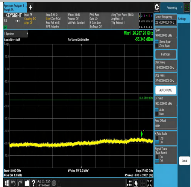
Band41-10MHz-QPSK-39700-1RB#0-18000~27000-PASS
