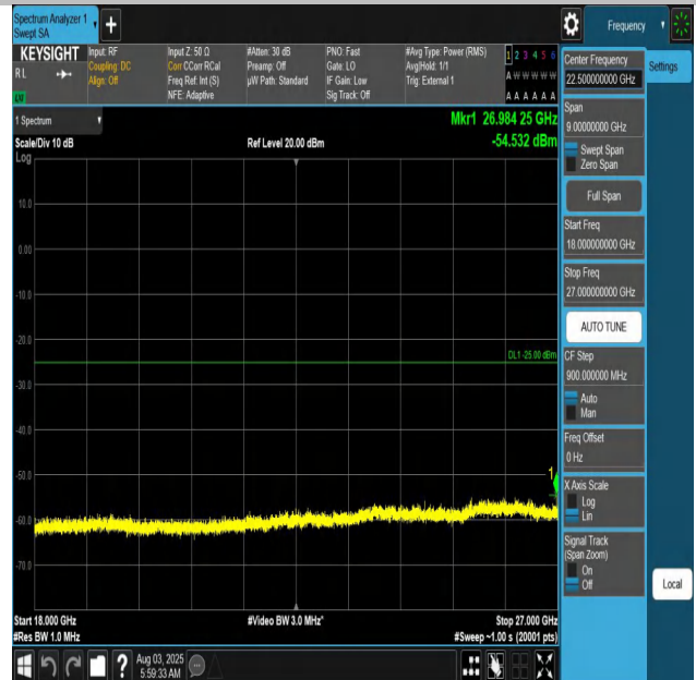
Band41-20MHz-QPSK-40620-1RB#0-18000~27000-PASS
