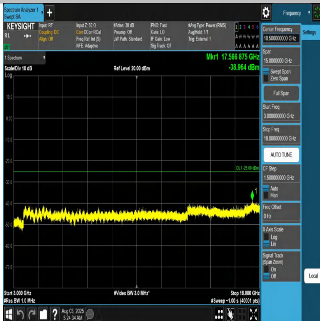
Band41-15MHz-QPSK-41515-1RB#0-3000~18000-PASS
