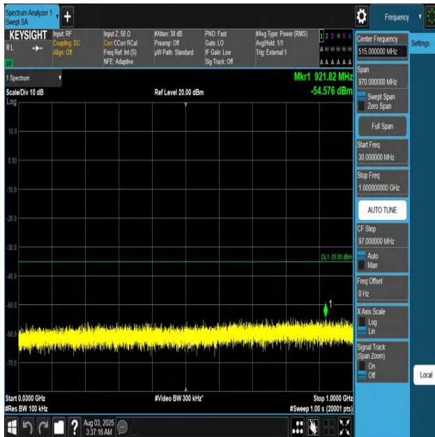
Band41-5MHz-QPSK-41565-1RB#0-30~1000-PASS
