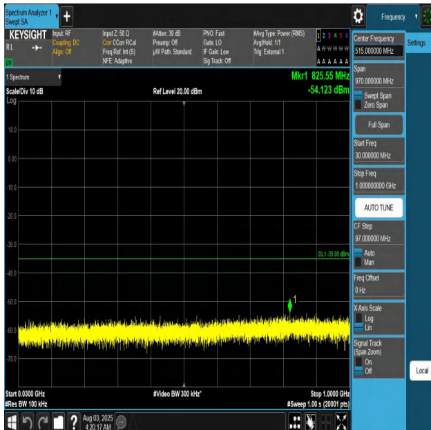
Band41-10MHz-QPSK-40620-1RB#0-30~1000-PASS
