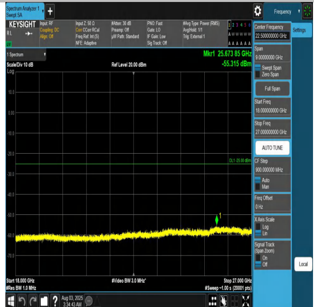
Band41-5MHz-QPSK-39675-1RB#0-18000~27000-PASS
