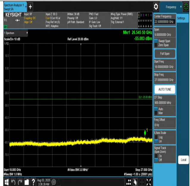
Band41-5MHz-QPSK-40620-1RB#0-18000~27000-PASS
