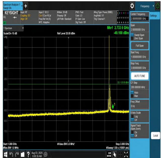
Band41-20MHz-QPSK-41490-1RB#0-1000~3000-PASS
