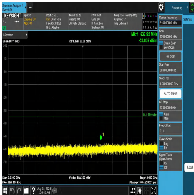
Band41-15MHz-QPSK-41515-1RB#0-30~1000-PASS
