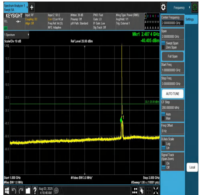
Band41-10MHz-QPSK-39700-1RB#0-1000~3000-PASS
