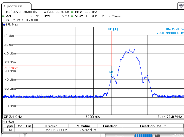
BLE_2M_Low_Channel
