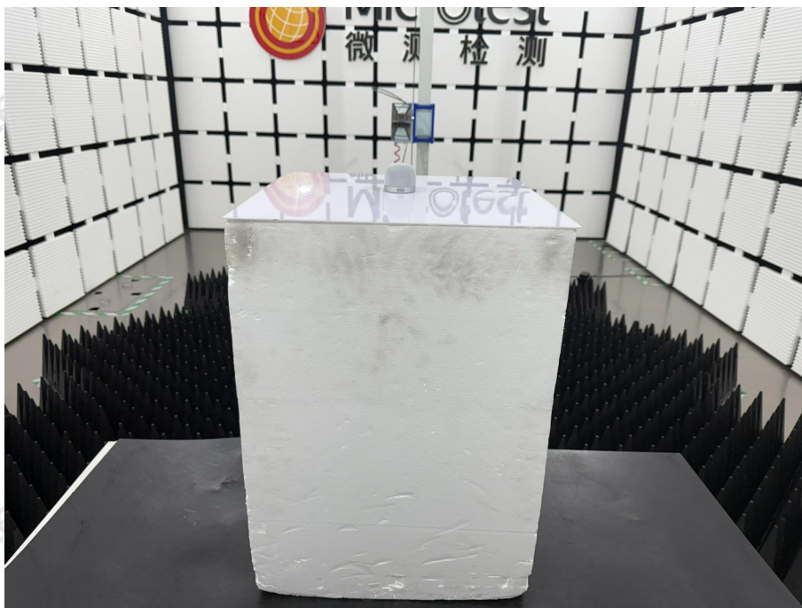
Radiated emissions (above 1GHz) -BT&BLE
