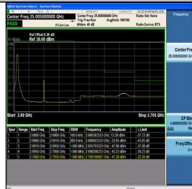
Band41-10MHz-16QAM-41540-1RB#49-PASS
