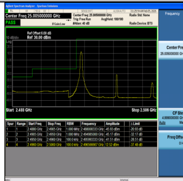
Band41-10MHz-QPSK-39700-1RB#49-PASS
