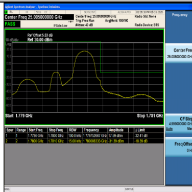
Band66-1.4MHz-64QAM-132665-1RB#5-PASS
