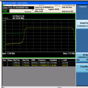
Band66-3MHz-16QAM-132657-1RB#0-PASS
