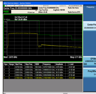
Band41-15MHz-64QAM-41515-75RB#0-PASS
