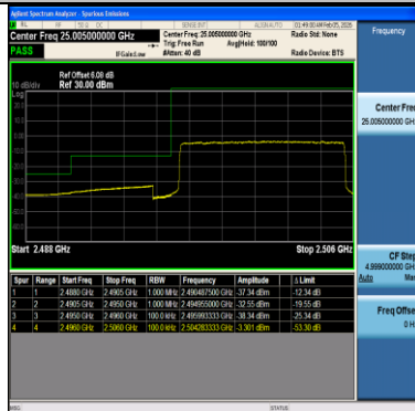
Band41-10MHz-64QAM-39700-50RB#0-PASS
