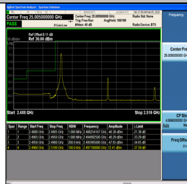
Band41-20MHz-16QAM-39750-1RB#0-PASS
