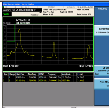
Band66-10MHz-QPSK-132022-1RB#0-PASS
