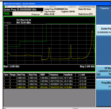
Band41-10MHz-64QAM-39700-1RB#49-PASS
