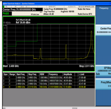
Band41-15MHz-QPSK-39725-75RB#0-PASS
