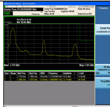
Band66-5MHz-64QAM-132647-1RB#0-PASS
