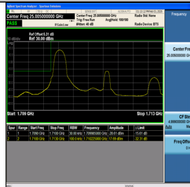
Band66-3MHz-QPSK-131987-1RB#14-PASS
