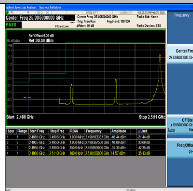
Band41-15MHz-QPSK-39725-1RB#74-PASS
