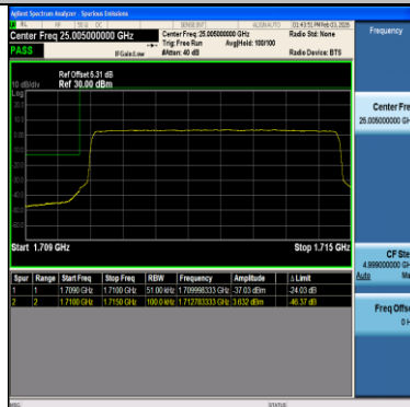
Band66-5MHz-64QAM-131997-25RB#0-PASS
