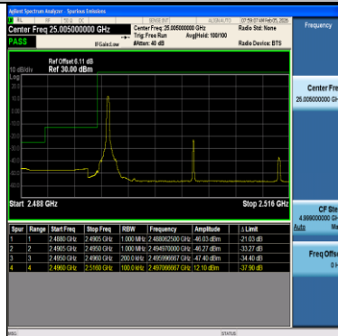
Band41-20MHz-16QAM-39750-1RB#99-PASS
