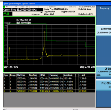
Band41-20MHz-QPSK-41490-100RB#0-PASS
