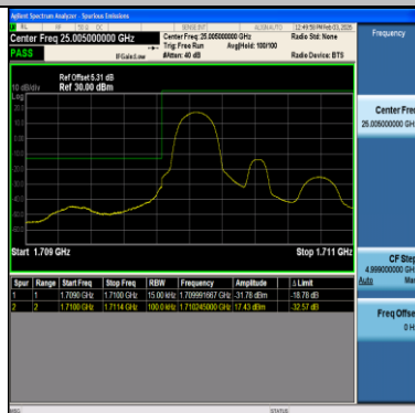
Band66-1.4MHz-16QAM-131979-1RB#5-PASS
