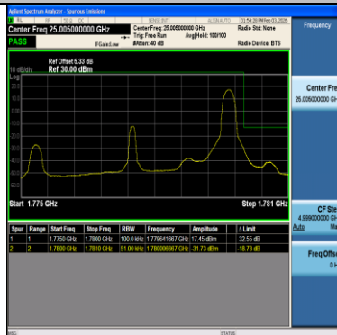
Band66-5MHz-16QAM-132647-25RB#0-PASS
