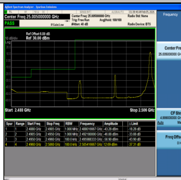
Band41-10MHz-16QAM-39700-1RB#49-PASS
