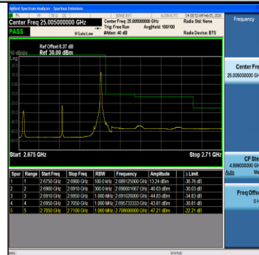
Band41-15MHz-QPSK-41515-75RB#0-PASS
