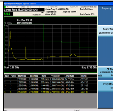
Band41-10MHz-64QAM-41540-1RB#0-PASS
