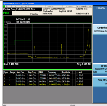
Band41-20MHz-64QAM-39750-1RB#99-PASS
