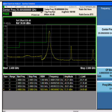
Band41-10MHz-64QAM-39700-1RB#0-PASS
