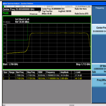
Band66-3MHz-64QAM-131987-15RB#0-PASS
