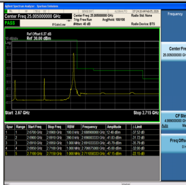
Band41-20MHz-16QAM-41490-100RB#0-PASS
