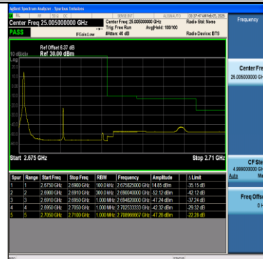
Band41-15MHz-64QAM-41515-1RB#0-PASS
