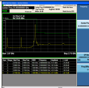
Band41-20MHz-64QAM-41490-1RB#99-PASS
