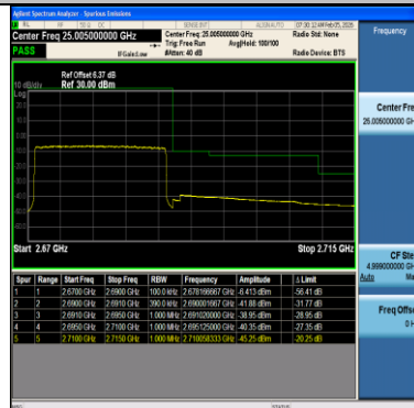
Band41-20MHz-64QAM-41490-100RB#0-PASS
