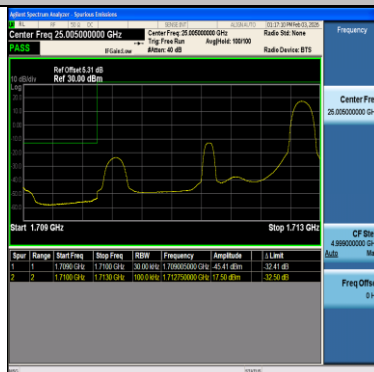
Band66-3MHz-16QAM-131987-1RB#14-PASS
