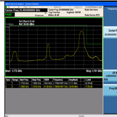
Band66-5MHz-QPSK-132647-25RB#0-PASS
