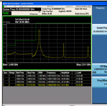
Band41-15MHz-64QAM-39725-1RB#0-PASS
