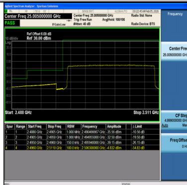
Band41-15MHz-64QAM-39725-75RB#0-PASS
