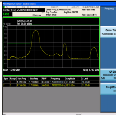
Band66-3MHz-64QAM-131987-1RB#0-PASS
