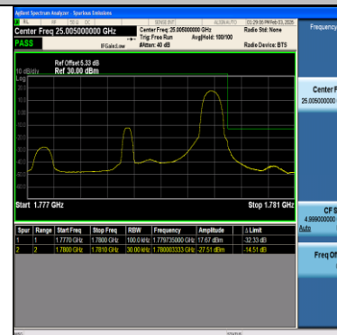
Band66-3MHz-16QAM-132657-1RB#14-PASS
