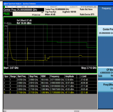
Band41-20MHz-16QAM-41490-1RB#99-PASS
