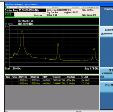
Band66-10MHz-16QAM-132022-1RB#0-PASS
