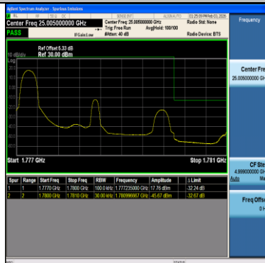
Band66-3MHz-QPSK-132657-1RB#14-PASS
