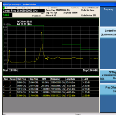
Band41-10MHz-QPSK-41540-1RB#49-PASS
