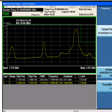
Band66-5MHz-64QAM-132647-1RB#24-PASS
