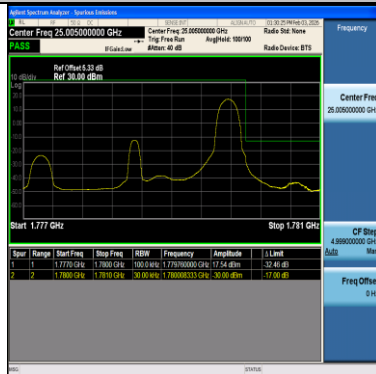
Band66-3MHz-16QAM-132657-15RB#0-PASS
