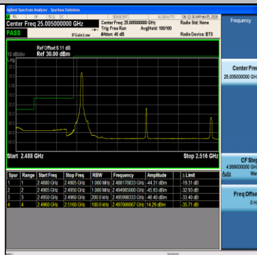
Band41-20MHz-QPSK-39750-1RB#0-PASS
