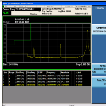
Band41-20MHz-QPSK-39750-100RB#0-PASS
