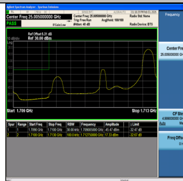
Band66-3MHz-64QAM-131987-1RB#14-PASS
