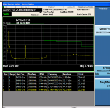
Band41-15MHz-16QAM-41515-1RB#0-PASS
