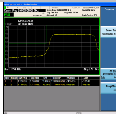
Band66-1.4MHz-16QAM-131979-6RB#0-PASS
