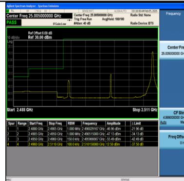
Band41-15MHz-16QAM-39725-75RB#0-PASS
