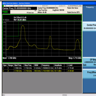
Band66-5MHz-64QAM-131997-1RB#0-PASS
