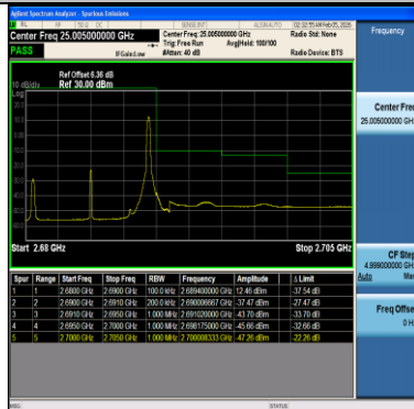
Band41-10MHz-16QAM-41540-50RB#0-PASS
