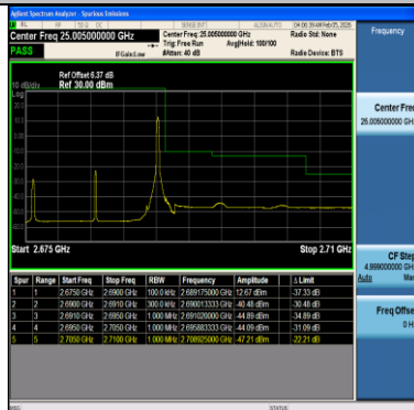
Band41-15MHz-16QAM-41515-75RB#0-PASS
