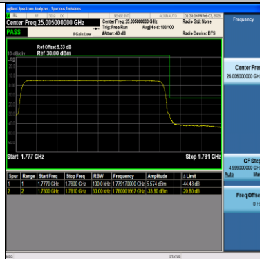
Band66-5MHz-QPSK-131997-1RB#0-PASS
