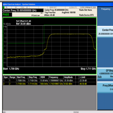
Band66-1.4MHz-QPSK-131979-6RB#0-PASS
