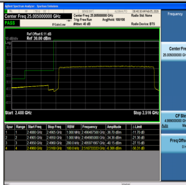
Band41-20MHz-64QAM-39750-100RB#0-PASS
