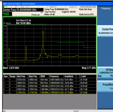
Band41-15MHz-64QAM-41515-1RB#74-PASS
