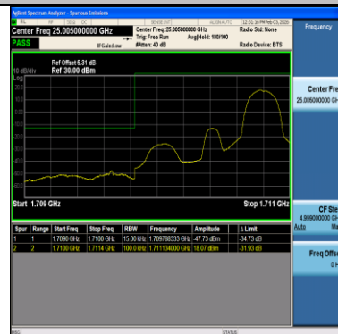
Band66-1.4MHz-64QAM-131979-1RB#5-PASS
