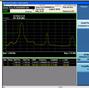
Band66-5MHz-QPSK-131997-1RB#24-PASS
