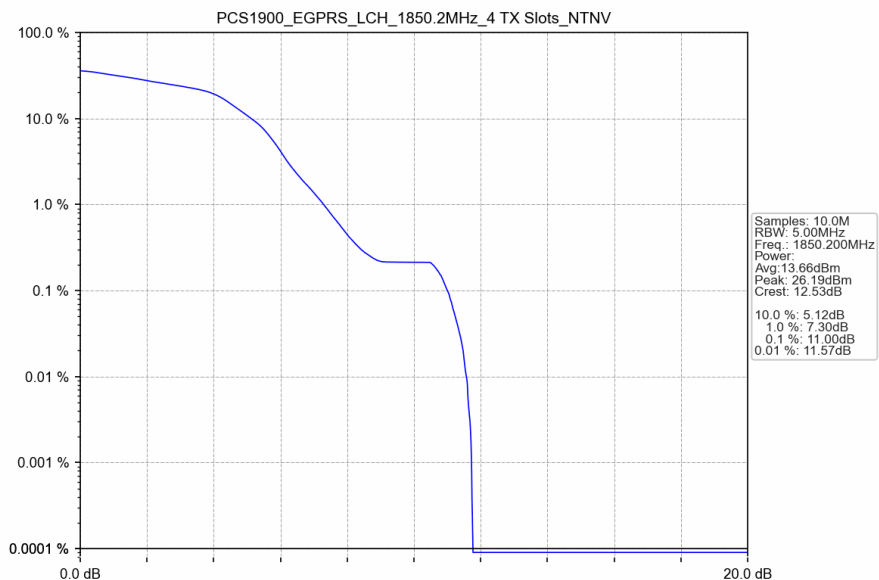
PCS1900_EGPRS_LCH_1850.2MHz_4 TX Slots_NTNV
