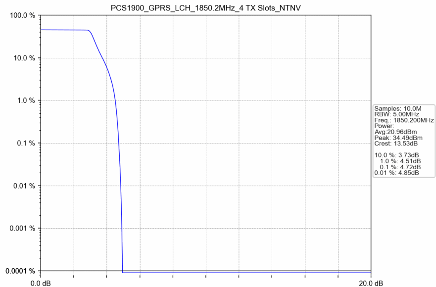
PCS1900_GPRS_LCH_1850.2MHz_4 TX Slots_NTNV
