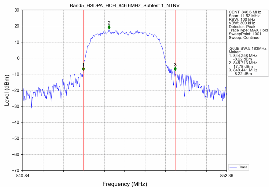
Band5_HSDPA_HCH_846.6MHz_Subtest 1_NTNV
