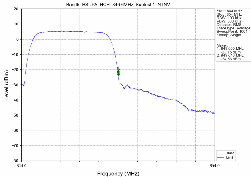
Band5_HSUPA_HCH_846.6MHz_Subtest 1_NTNV
