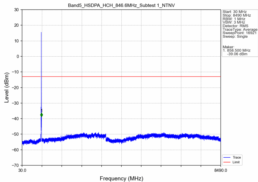
Band5_HSDPA_HCH_846.6MHz_Subtest 1_NTNV
