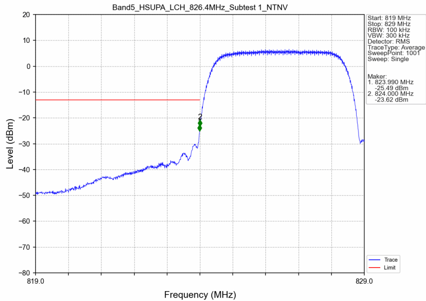
Band5_HSUPA_LCH_826.4MHz_Subtest 1_NTNV
