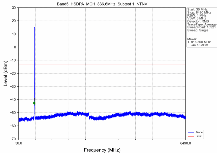
Band5_HSDPA_MCH_836.6MHz_Subtest 1_NTNV
