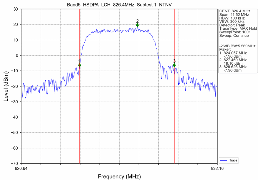
Band5_HSDPA_LCH_826.4MHz_Subtest 1 NTN
