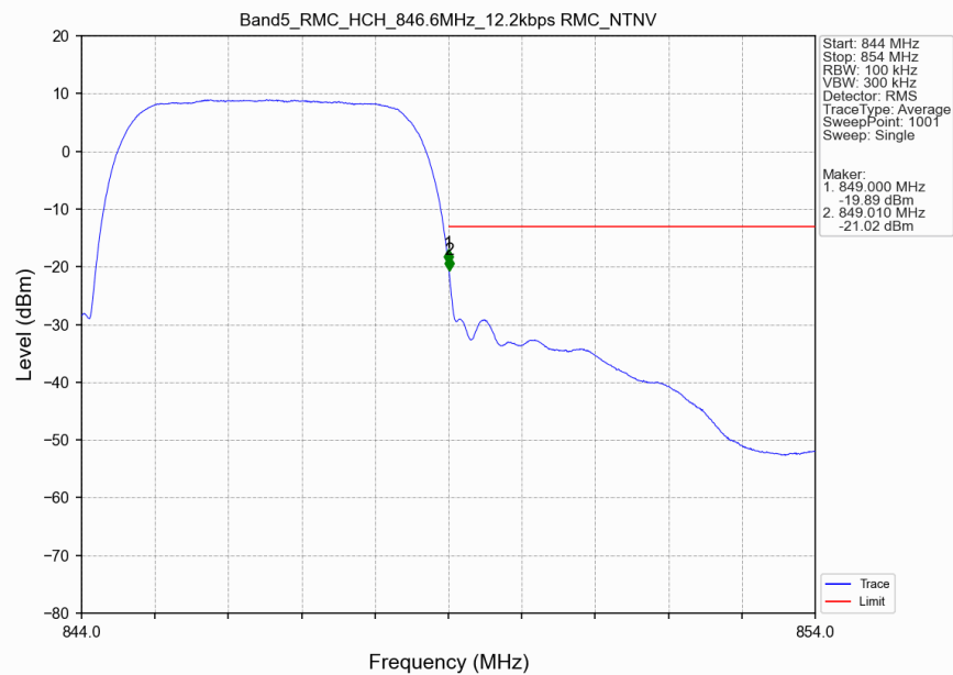
Band5_RMC_HCH_846.6MHz_12.2kbps RMC_NTNV
