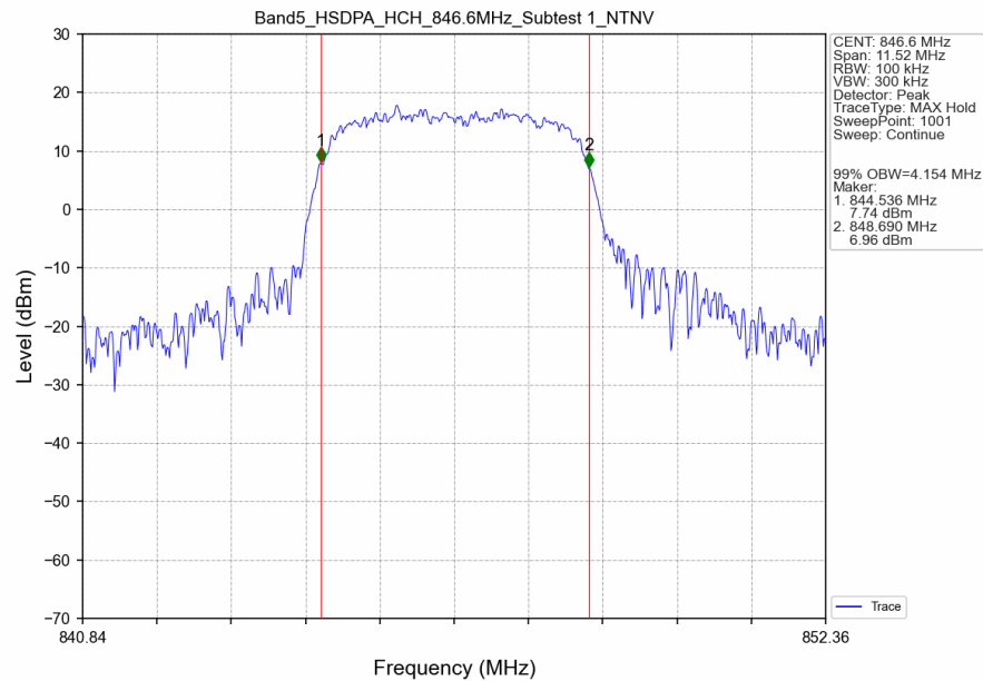
Band5_HSDPA_HCH_846.6MHz_Subtest 1_NTNV
