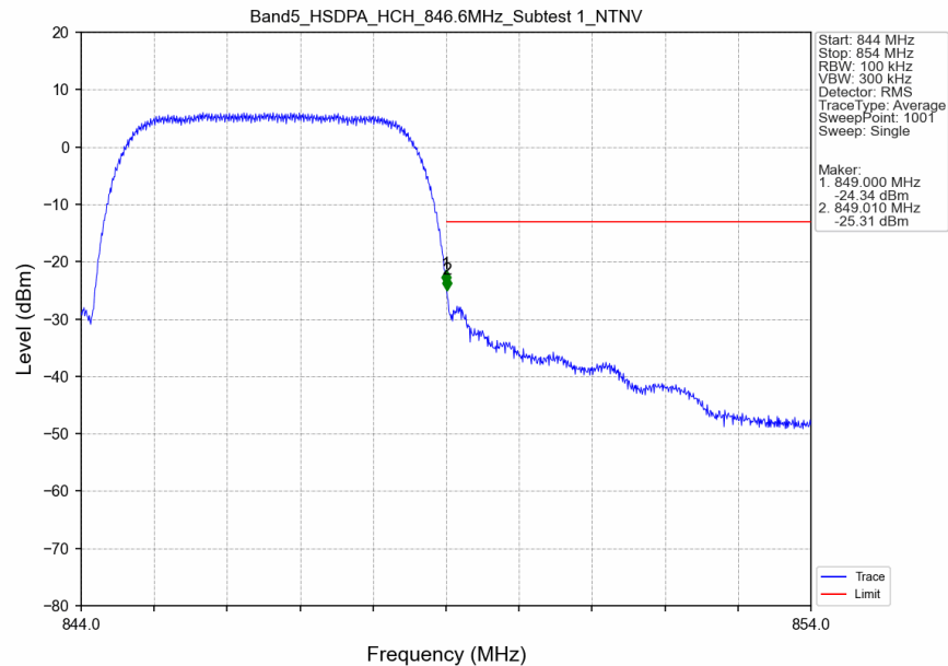
Band5_HSDPA_HCH_846.6MHz_Subtest 1_NTNV
