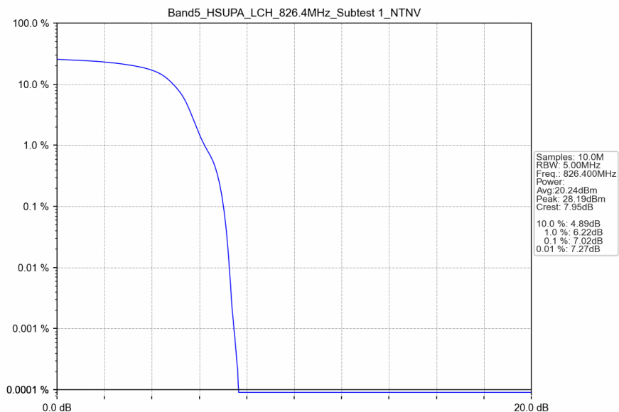
Band5_HSUPA_LCH_826.4MHz_Subtest 1_NTNV
