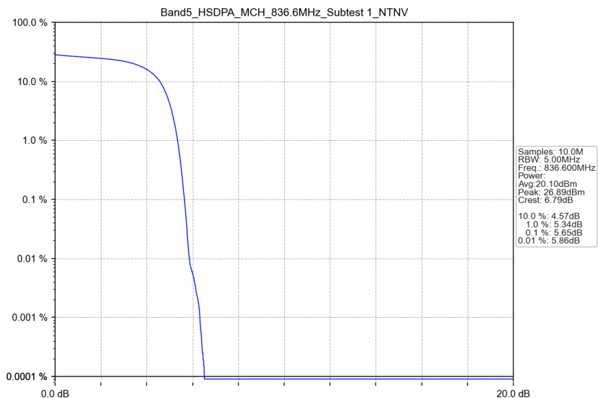
Band5_HSDPA_MCH_836.6MHz_Subtest 1_NTNV
