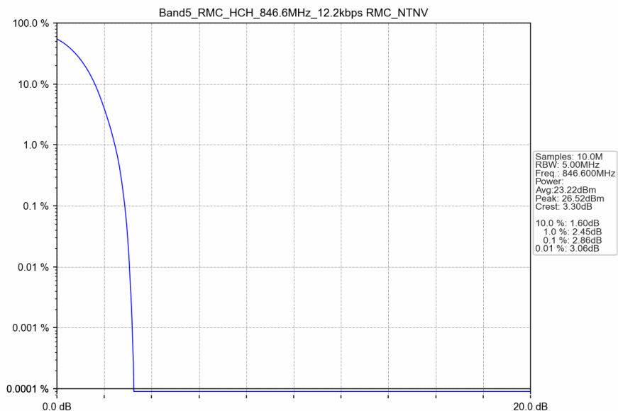
Band5_RMC_HCH_846.6MHz_12.2kbps RMC_NTNV
