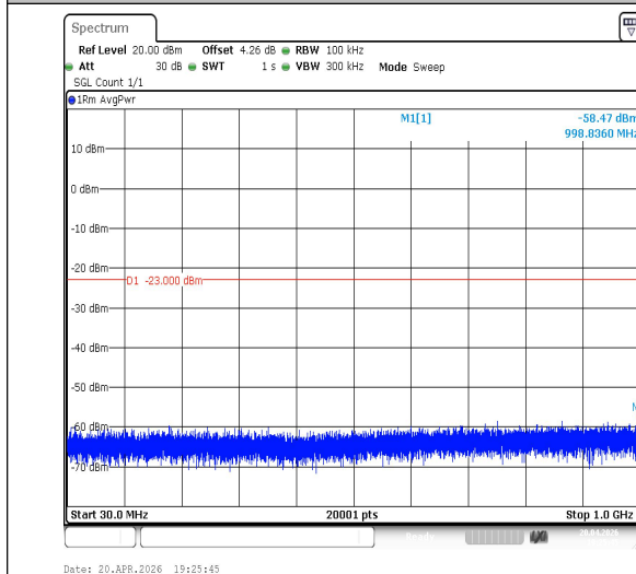
Band2-1.4MHz-QPSK-19193-1RB#0-30~1000-PASS
