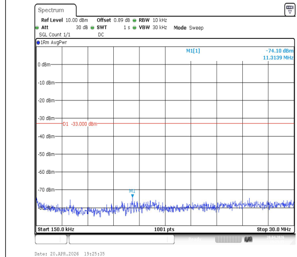
Band2-1.4MHz-QPSK-19193-1RB#0-0.15~30-PASS
