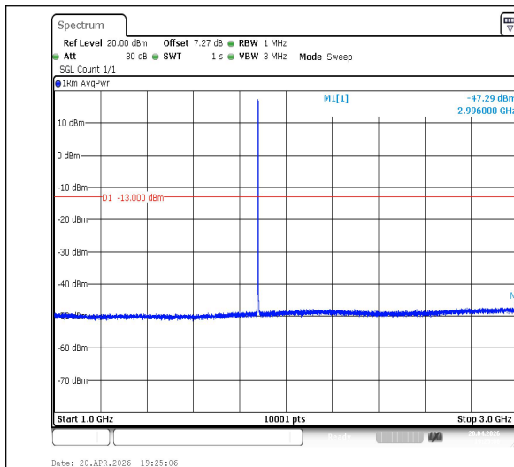
Band2-1.4MHz-16QAM-18900-1RB#0-1000~3000-PASS
