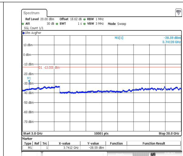
Band2-1.4MHz-16QAM-18900-1RB#0-3000~20000-PASS
