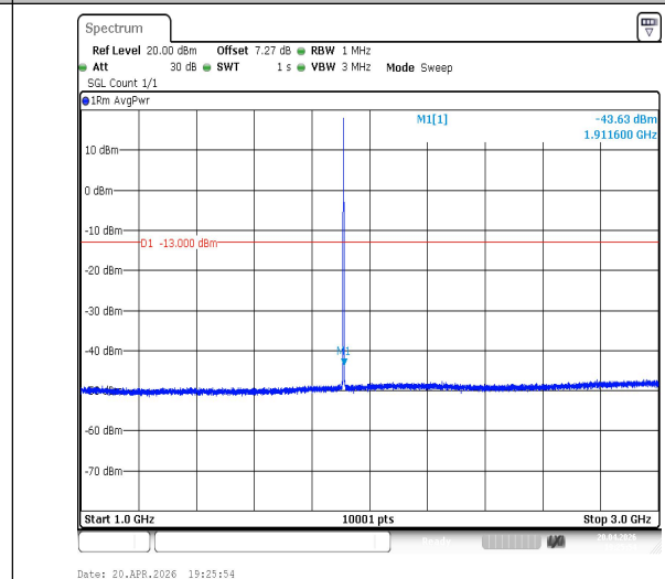
Band2-1.4MHz-QPSK-19193-1RB#0-1000~3000-PASS
