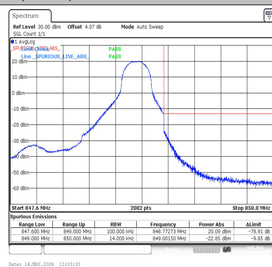
26(824-849)-1.4MHz-QPSK-27033-1RB#5-PASS
