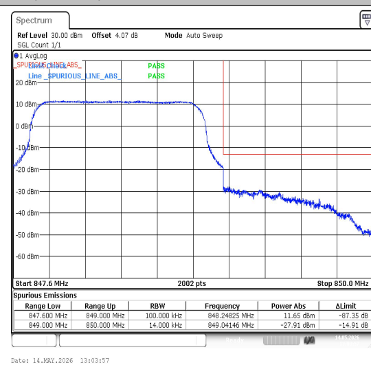
26(824-849)-1.4MHz-QPSK-27033-6RB#0-PASS
