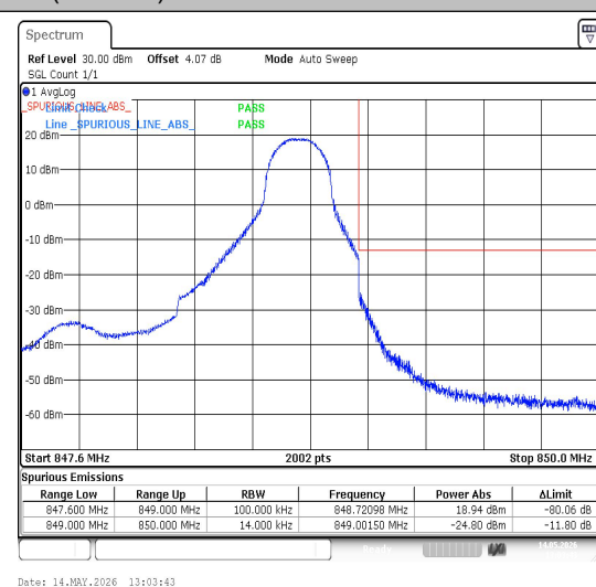
26(824-849)-1.4MHz-16QAM-27033-1RB#5-PASS
