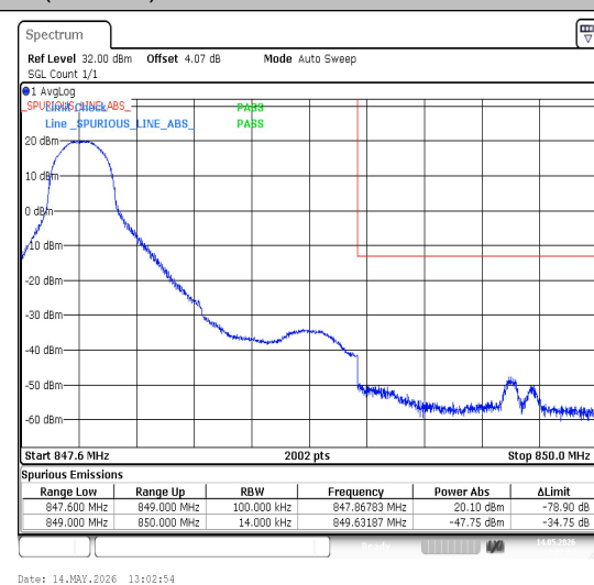
26(824-849)-1.4MHz-QPSK-27033-1RB#0-PASS
