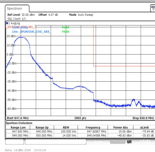
26(824-849)-1.4MHz-16QAM-27033-1RB#0-PASS
