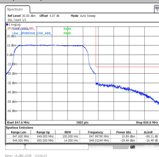
26(824-849)-1.4MHz-16QAM-27033-6RB#0-PASS
