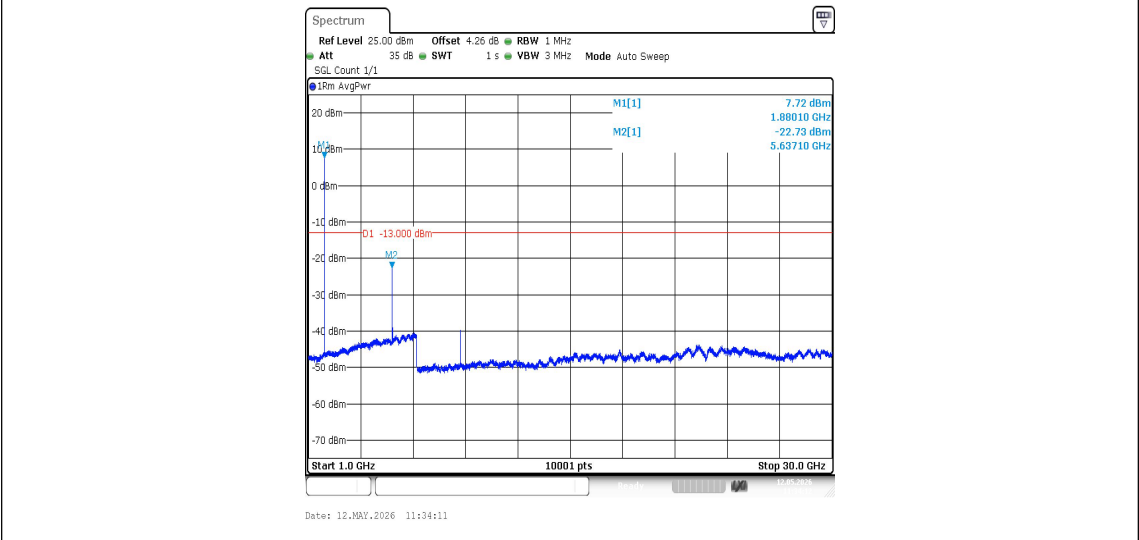
Band2-9400-2-1000~30000MHz-PASS
