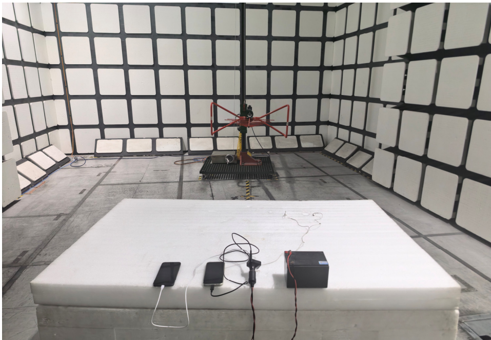
Radiated Emissions View (Below 1 GHz)
