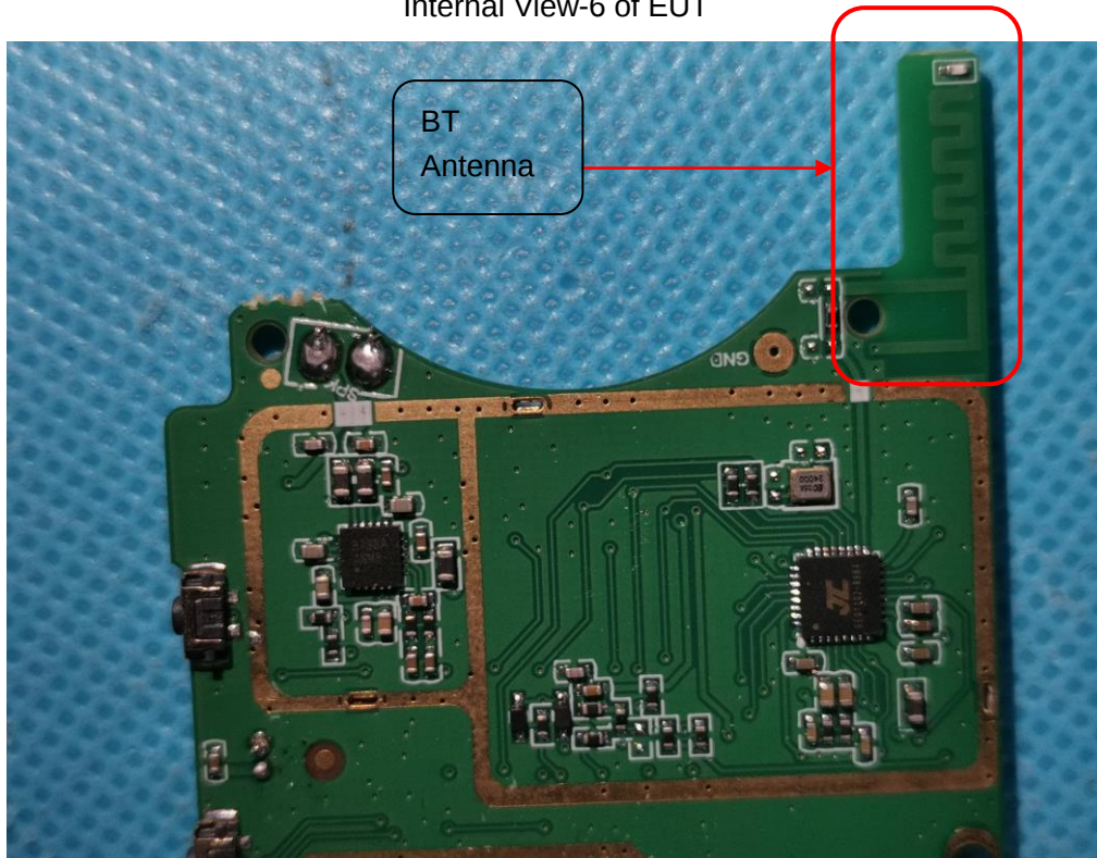
Internal View-6 of EUT
