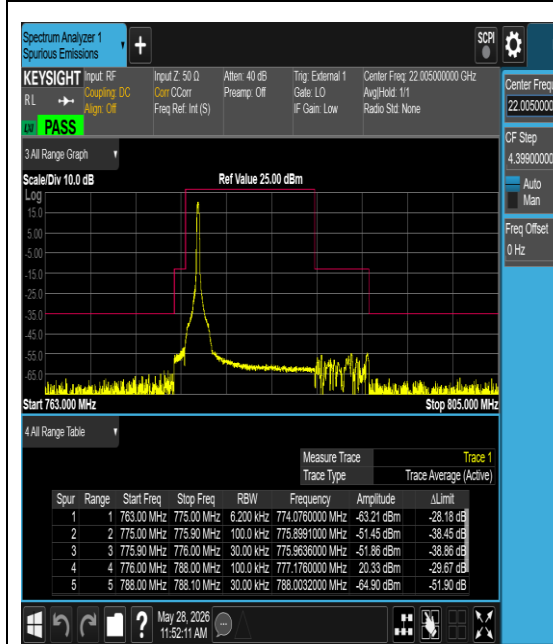
Band13-0.18-QPSK-23182-12@0-15kHz-PASS
