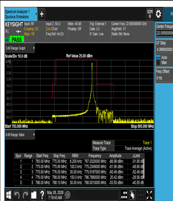
Band13-0.18-QPSK-23278-12@0-15kHz-PASS
