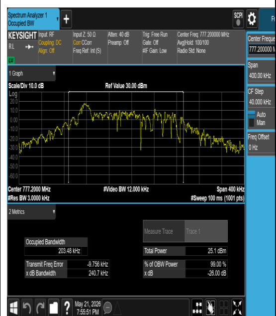
Band13-0.18-BPSK-23182-12@0-15kHz-PASS
