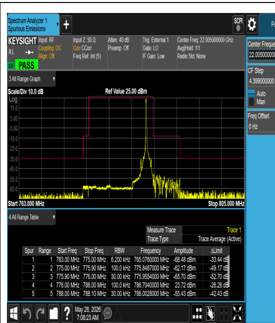
Band13-0.18-QPSK-23278-1@0-15kHz-PASS
