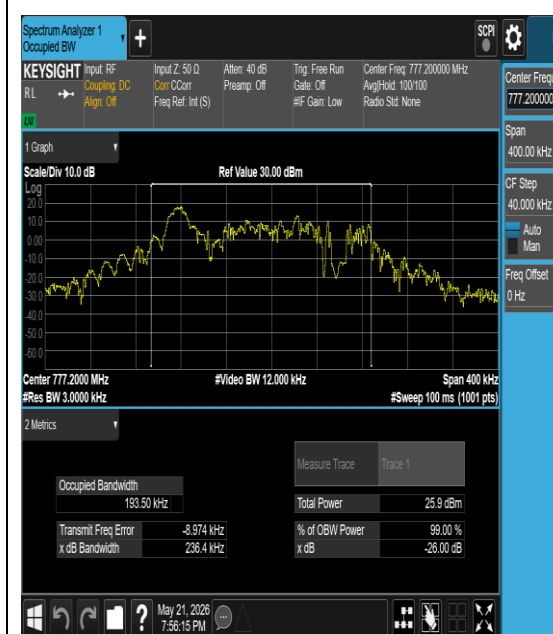
Band13-0.18-QPSK-23182-12@0-15kHz-PASS
