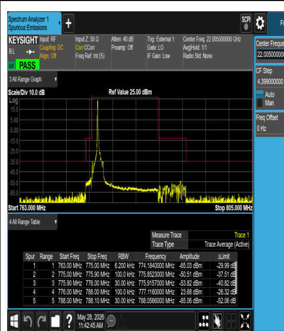
Band13-0.18-BPSK-23182-1@0-15kHz-PASS
