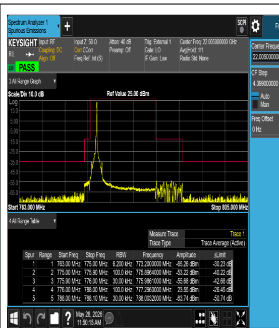
Band13-0.18-QPSK-23182-1@11-15kHz-PASS
