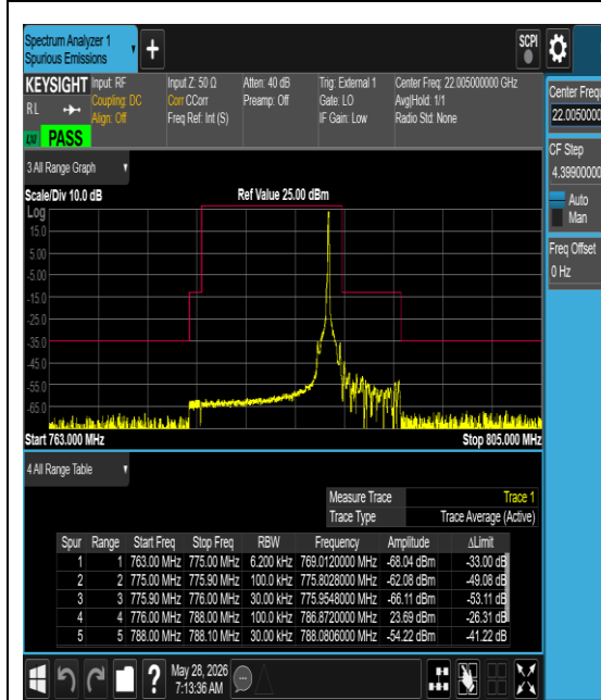
Band13-0.18-QPSK-23278-1@11-15kHz-PASS
