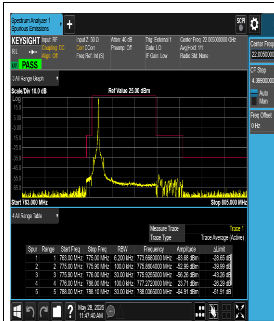
Band13-0.18-BPSK-23182-1@11-15kHz-PASS
