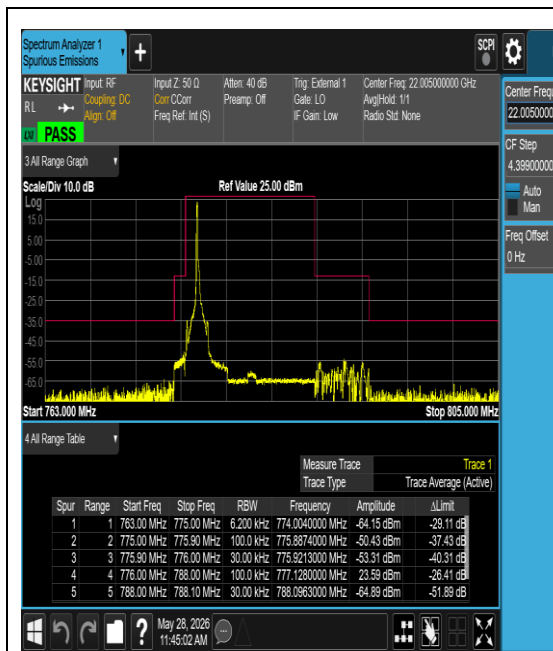
Band13-0.18-QPSK-23182-1@0-15kHz-PASS
