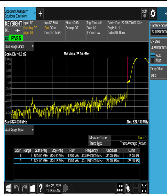
Band5-0.18-BPSK-20402-1@0-15kHz-PASS
