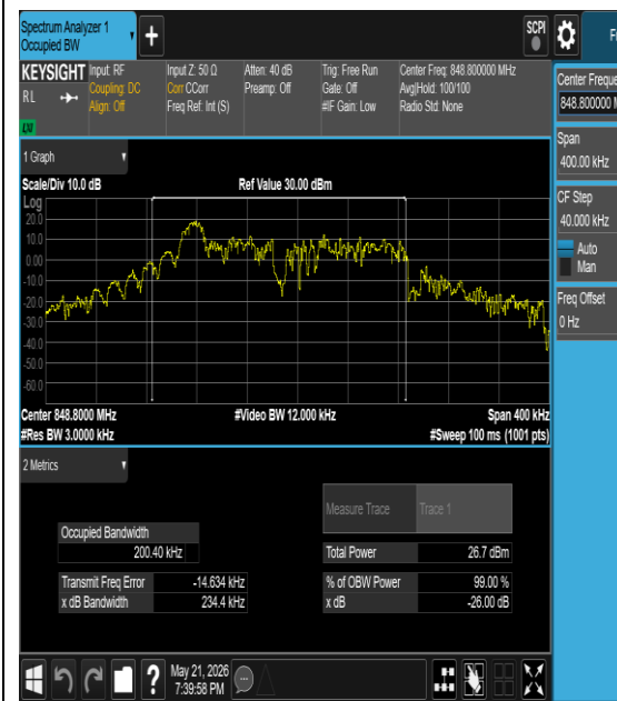
Band5-0.18-QPSK-20648-12@0-15kHz-PASS
