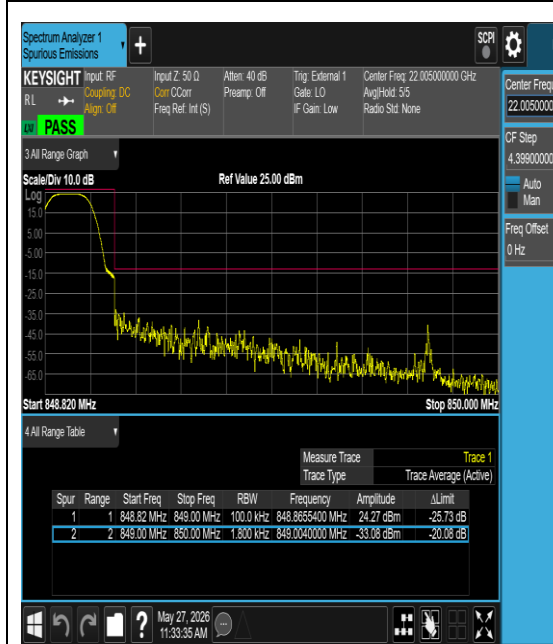
Band5-0.18-QPSK-20648-1@11-15kHz-PASS
