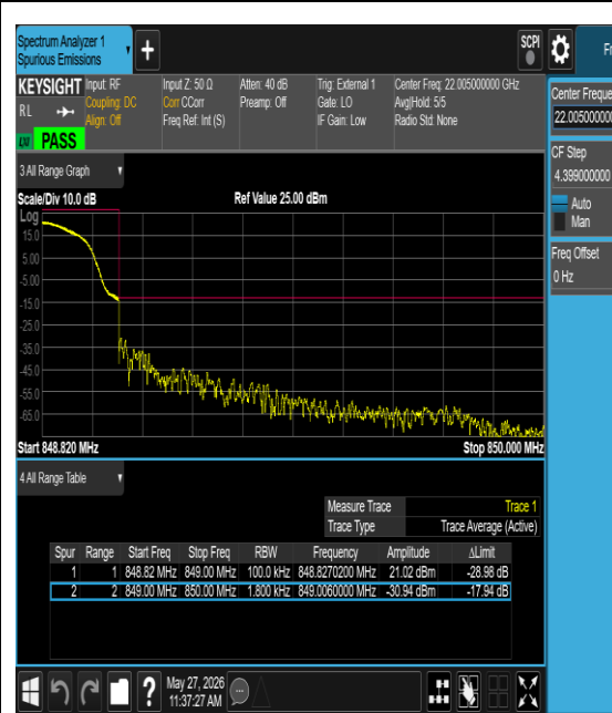
Band5-0.18-QPSK-20648-12@0-15kHz-PASS
