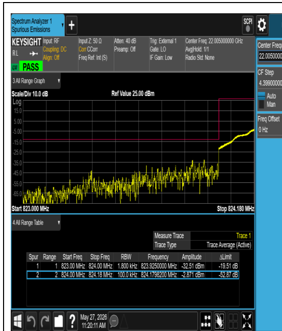
Band5-0.18-BPSK-20402-1@11-15kHz-PASS
