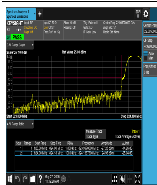
Band5-0.18-QPSK-20402-1@0-15kHz-PASS
