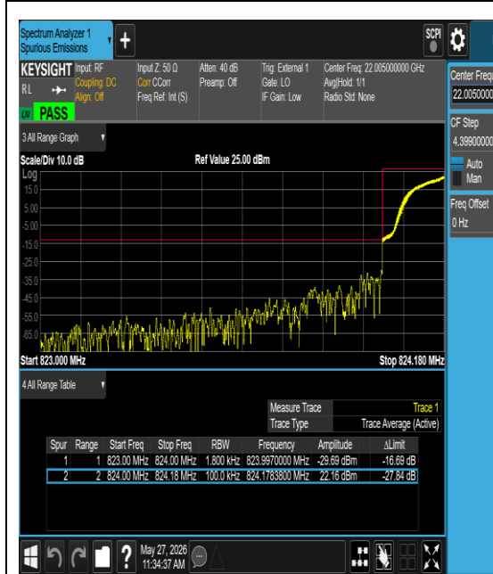
Band5-0.18-QPSK-20402-12@0-15kHz-PASS
