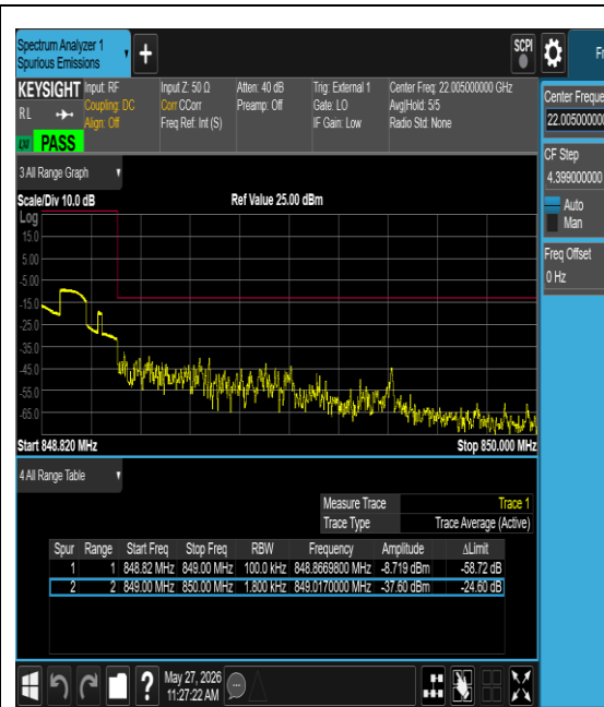
Band5-0.18-QPSK-20648-1@0-15kHz-PASS
