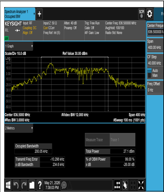
Band5-0.18-BPSK-20525-12@0-15kHz-PASS
