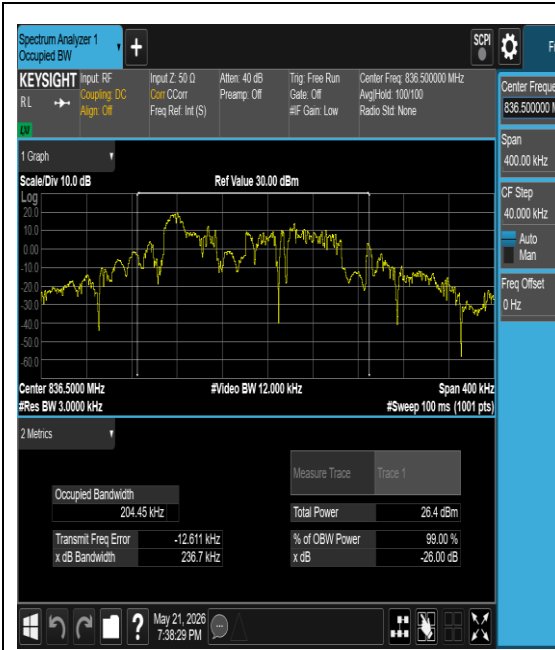
Band5-0.18-QPSK-20525-12@0-15kHz-PASS
