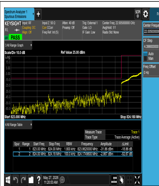
Band5-0.18-QPSK-20402-1@11-15kHz-PASS
