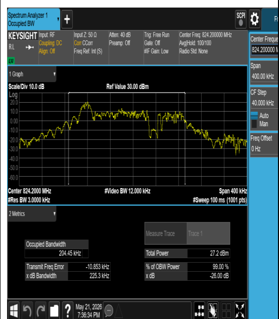
Band5-0.18-BPSK-20402-12@0-15kHz-PASS
