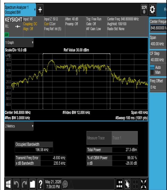
Band5-0.18-BPSK-20648-12@0-15kHz-PASS
