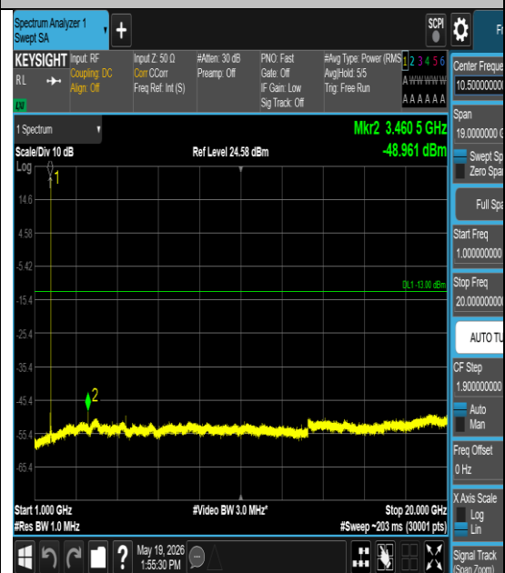
Band4-5MHz-16QAM-20175-1#0-1000-20000-PASS
