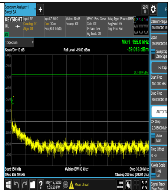
Band4-5MHz-16QAM-20175-1#0-0.15-30-PASS
