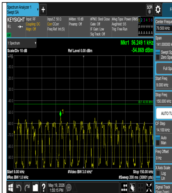
Band4-5MHz-16QAM-20175-1#0-0.009-0.15-PASS
