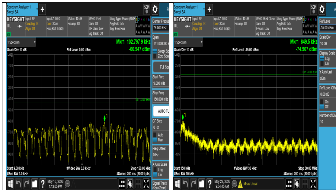
Band4-5MHz-QPSK-20175-1#0-0.009-0.15-PASS
