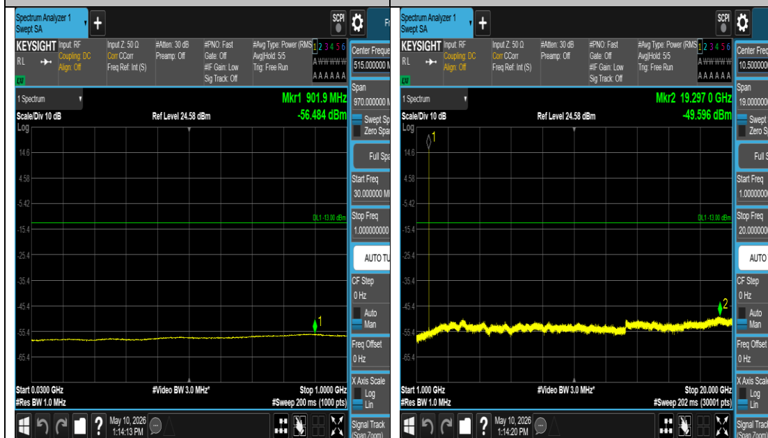
Band4-5MHz-QPSK-20375-1#5-1000-20000-PASS
