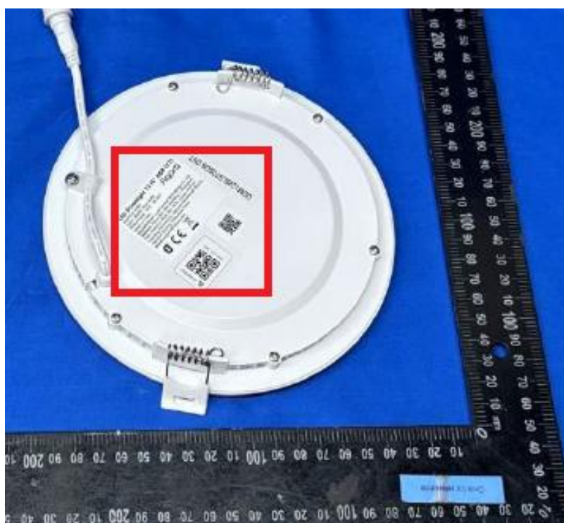
Label location
