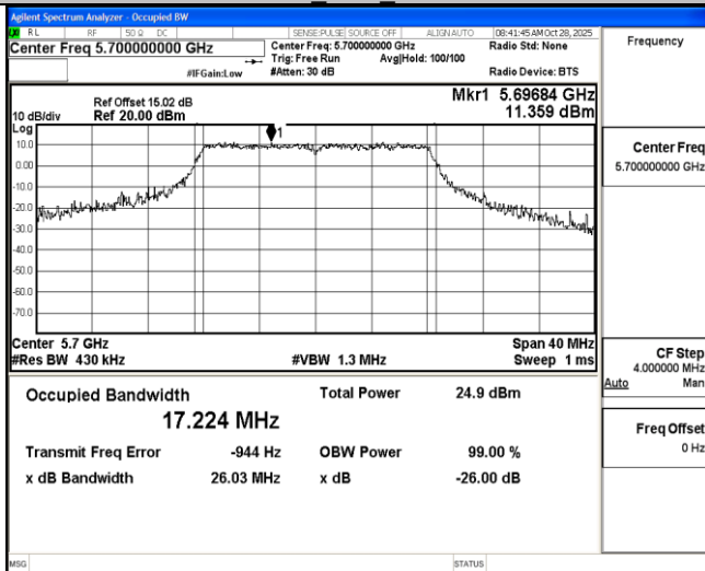
11A Ant2 5700
