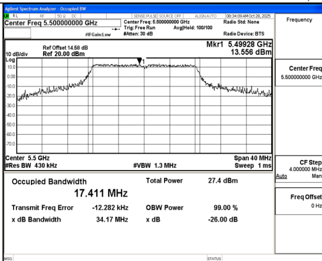
11A Ant2 5500
