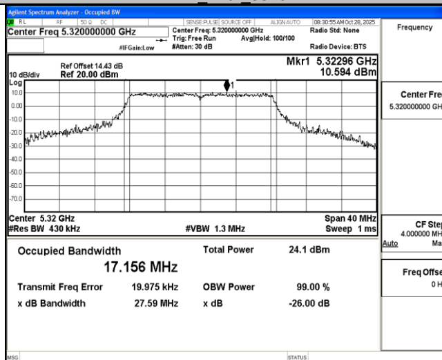
11A Ant2 5320
