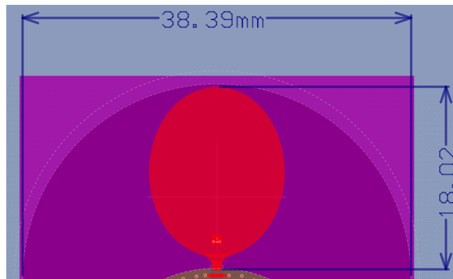
Figure 1: Antenna Dimensions
