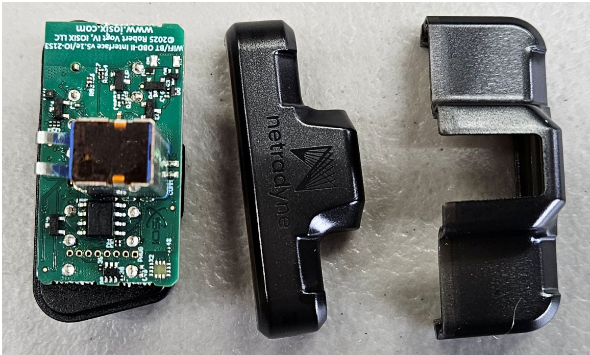
Internal Photo - Assembly - 1
