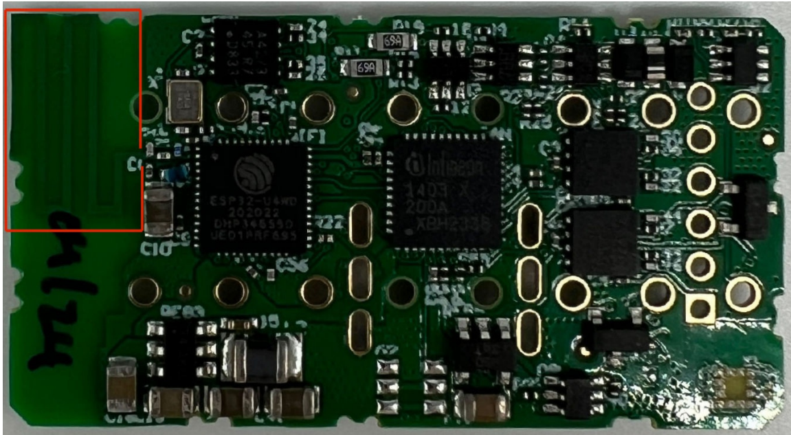
Internal Photo - PCB - Bottom - Radio Section
