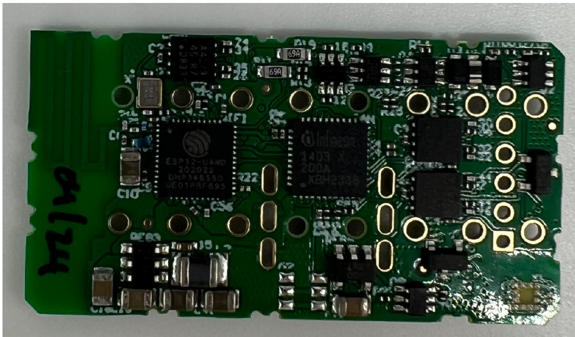
Internal Photo - PCB - Bottom
