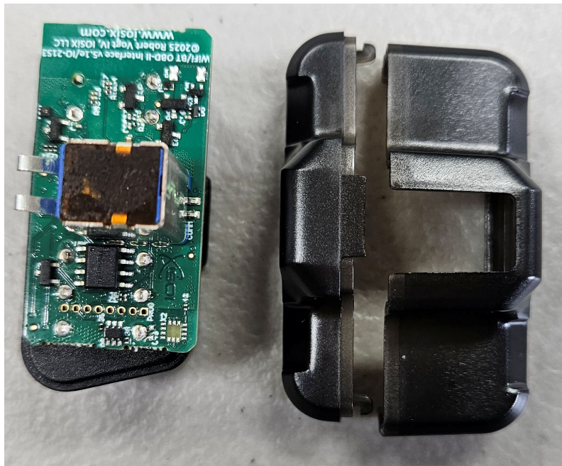
Internal Photo - Assembly - 2
