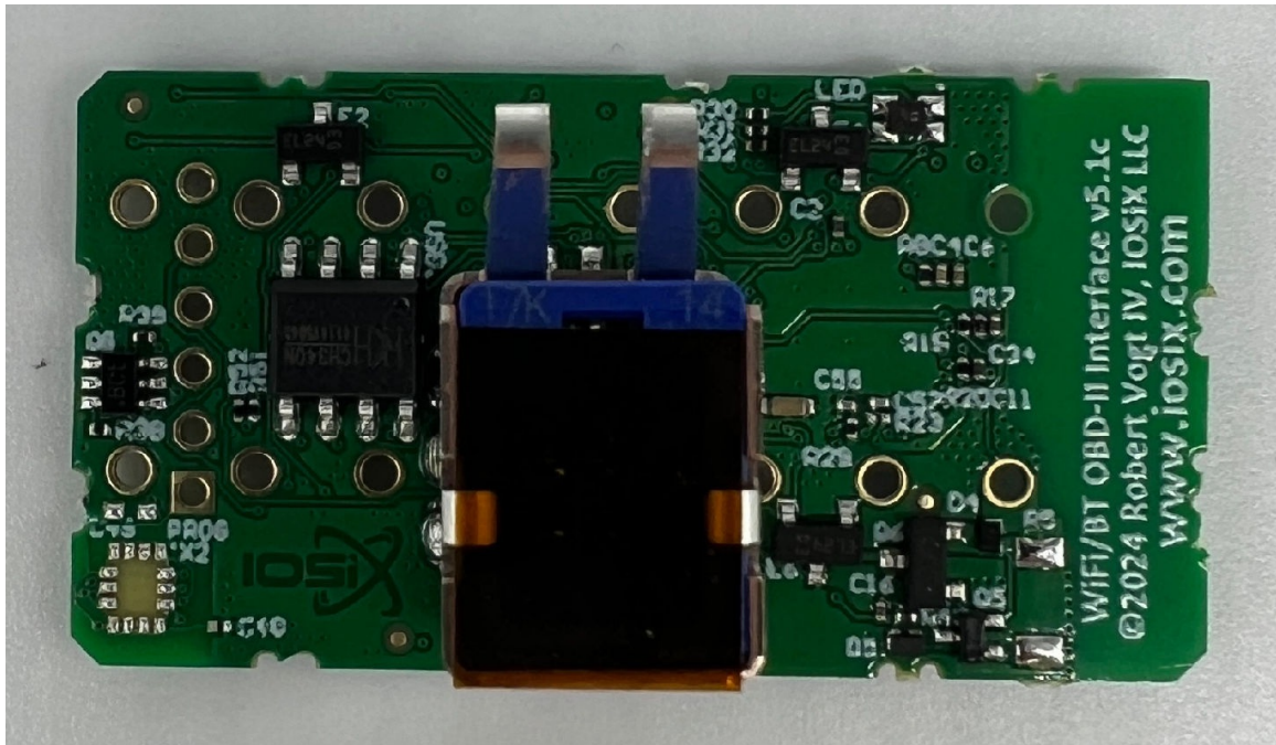
Internal Photo - PCB - Top
