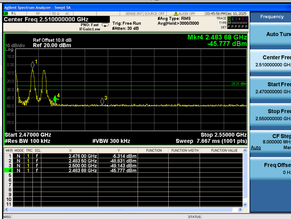
GFSK-Ant1-Hop_2480-PASS
