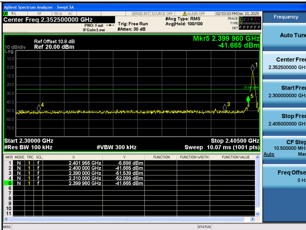
GFSK-Ant1-2402-PASS
