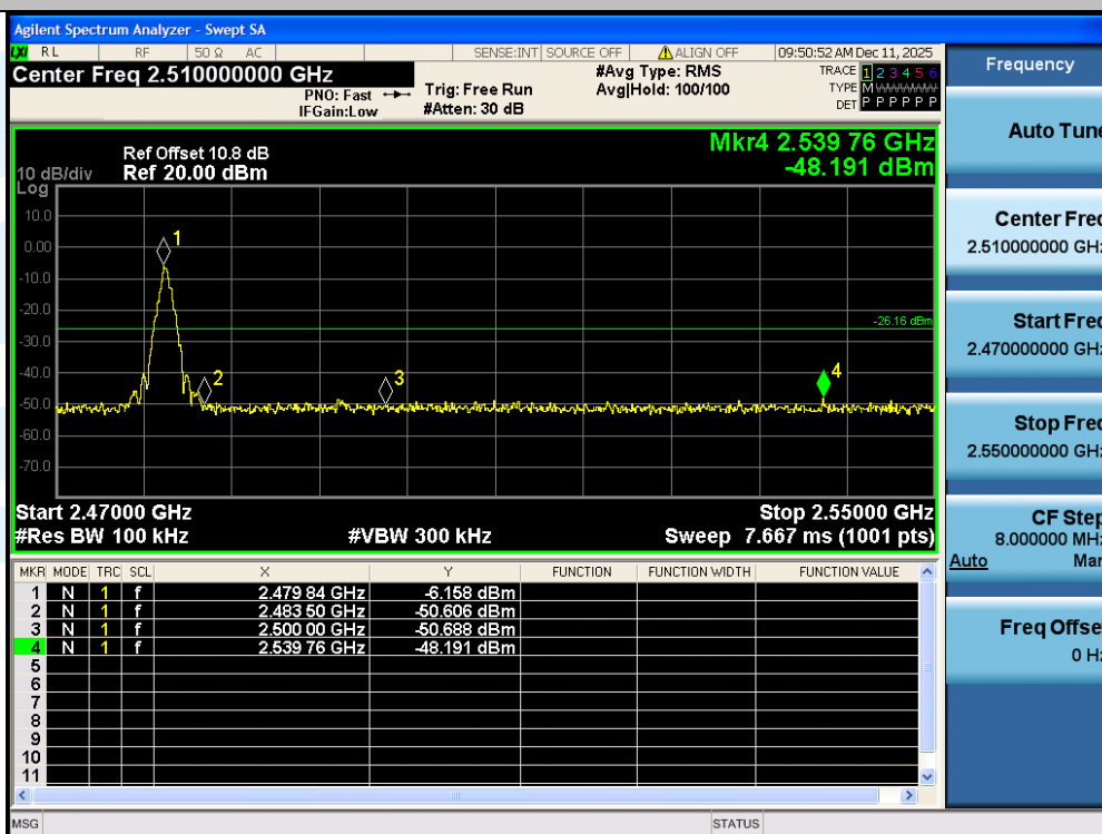
GFSK-Ant1-2480-PASS
