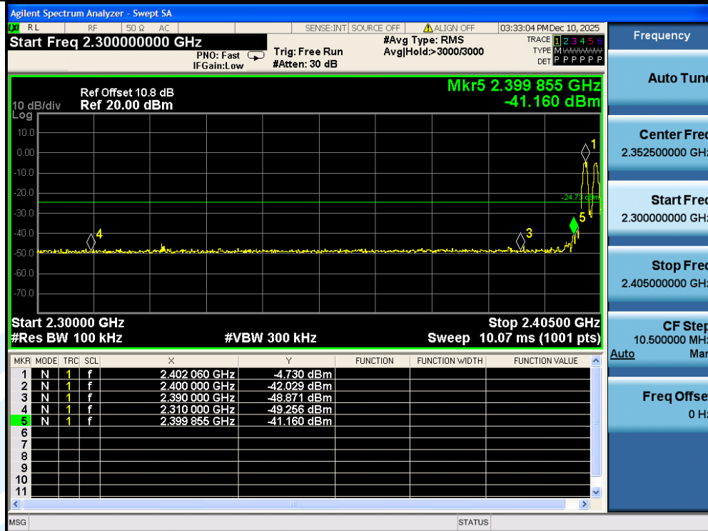
GFSK-Ant1-Hop_2402-PASS
