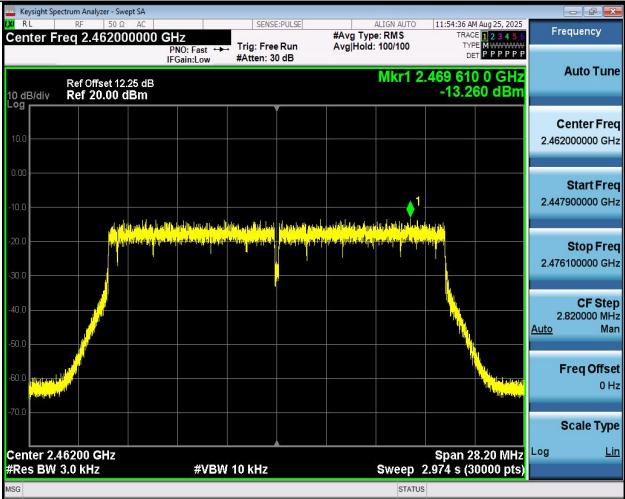
11BE20MIMO-Ant2-2462-PASS
