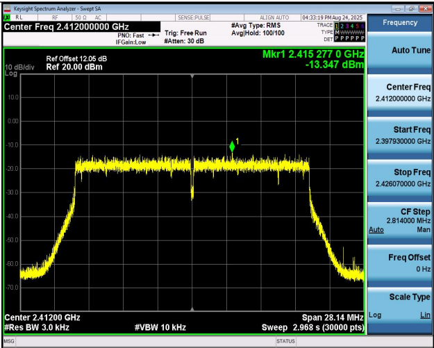
11AX20MIMO-Ant1-2412-PASS
