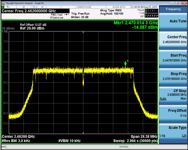
11BE20MIMO-Ant1-2462-PASS
