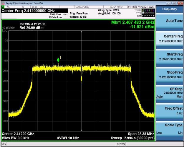
11AX20MIMO-Ant2-2412-PASS
