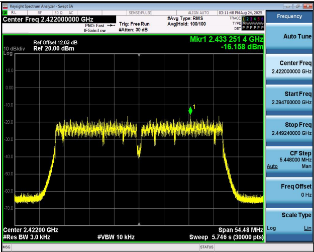
11N40MIMO-Ant1-2422-PASS
