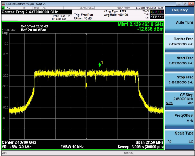
11BE20MIMO-Ant2-2437-PASS
