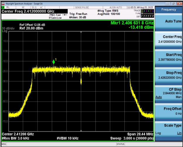
11BE20MIMO-Ant1-2412-PASS
