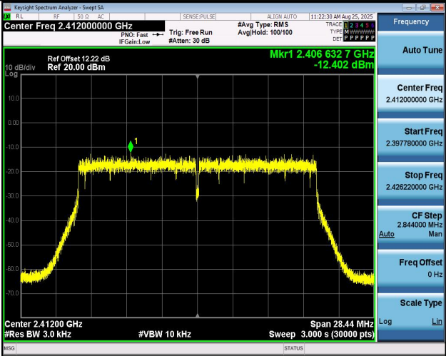
11BE20MIMO-Ant2-2412-PASS
