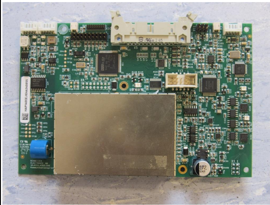
Radio PCB top view
