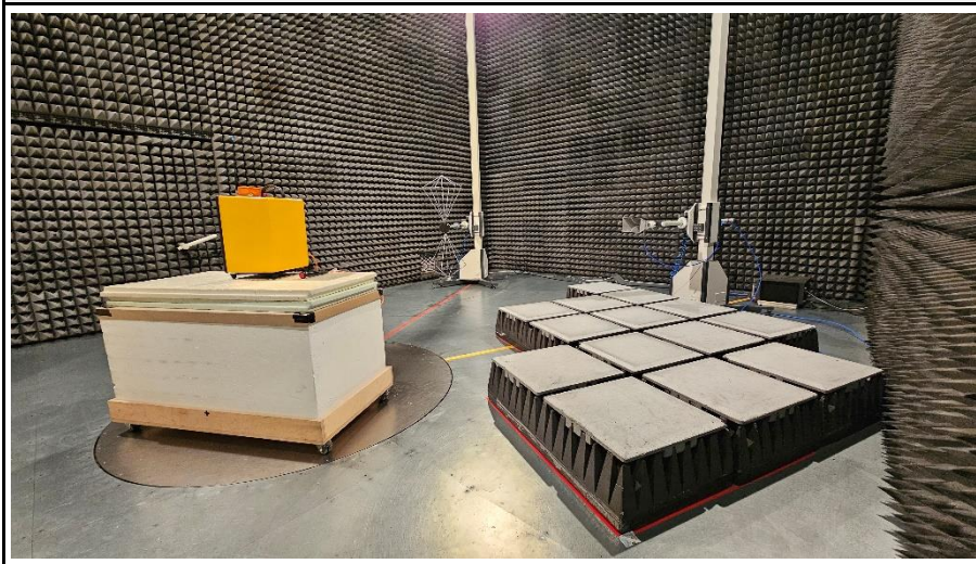
TEST SETUP Rx 30 MHz - 200 MHz
