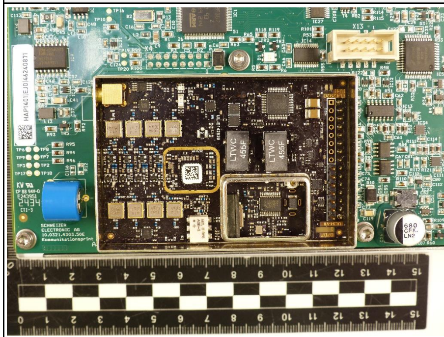
Radio PCB top view without all shielding
