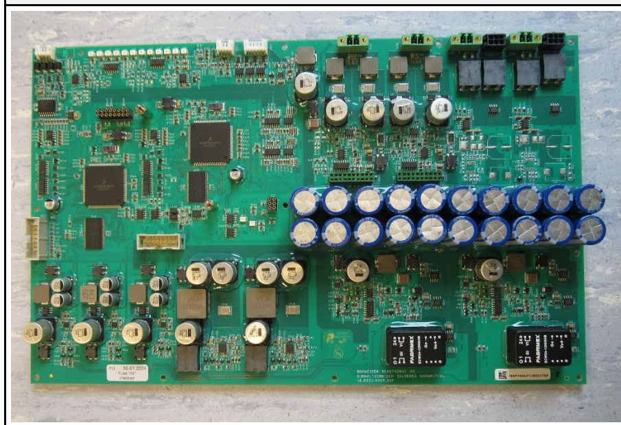
PCB2 top side
