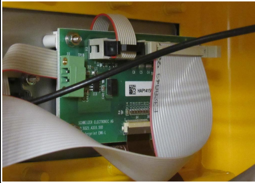
Display/Keyboard PCB top view
