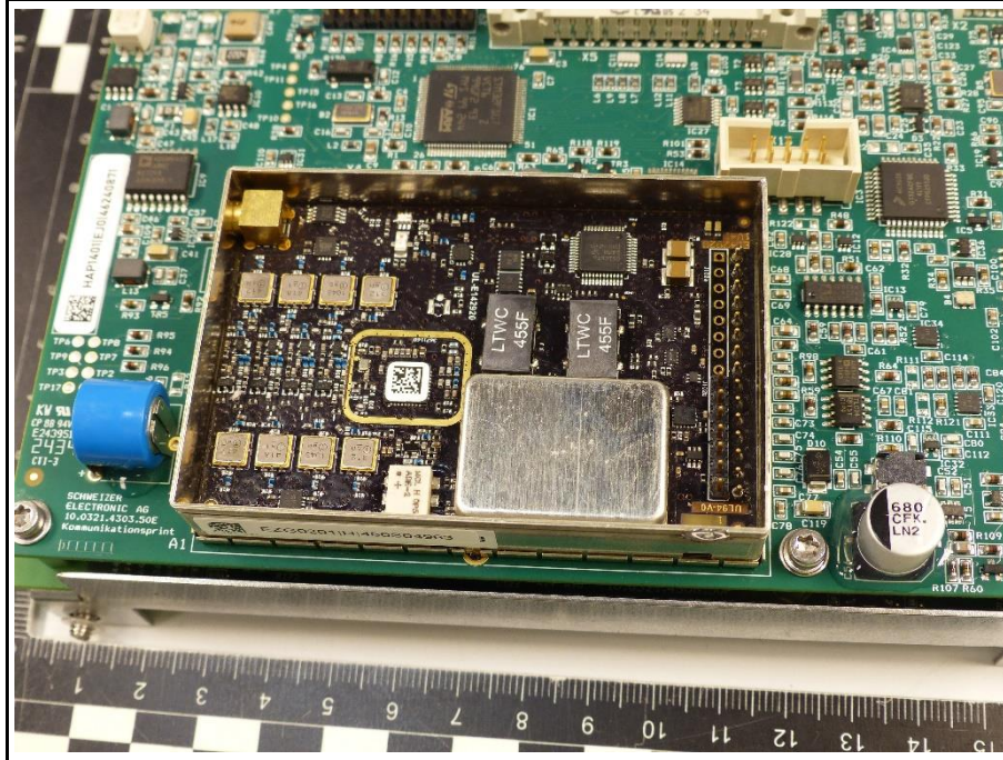
Radio PCB top view without main shielding
