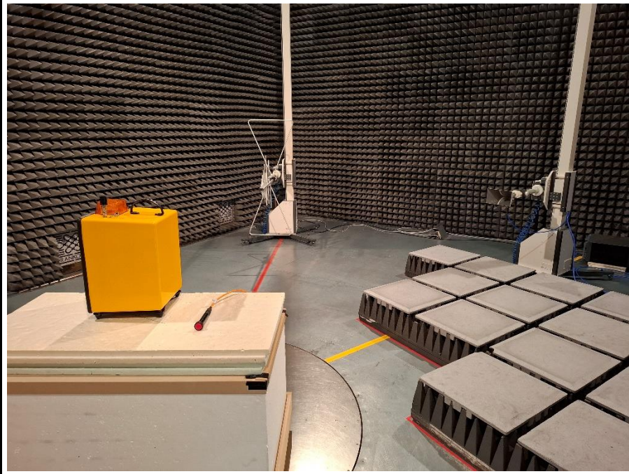
TEST SETUP Tx 30 MHz – 1 GHz
