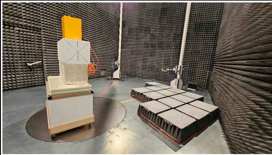
TEST SETUP Tx 1 GHz - 5 GHz
